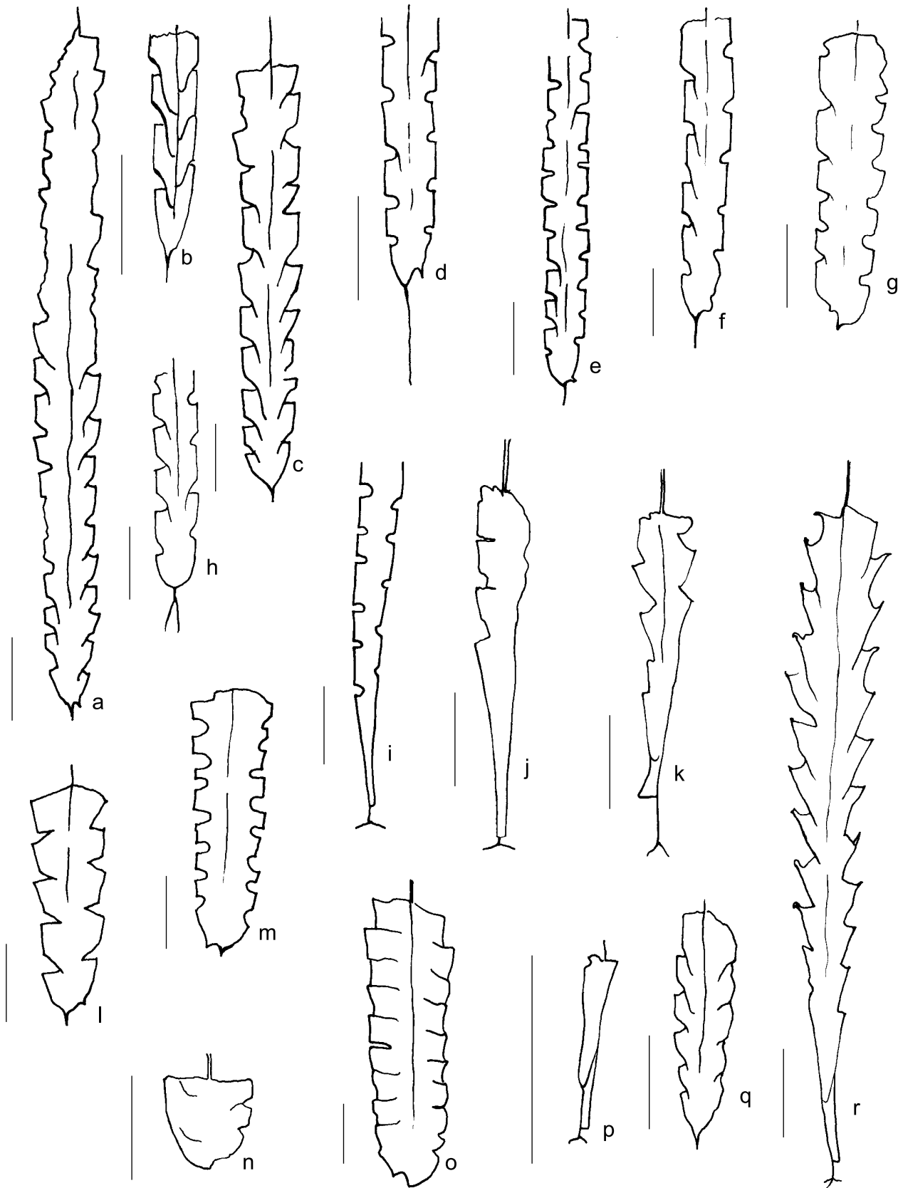
Fig. 4. a–c — Normalograptus cf. persculptus (Elles and Wood), sample BS. 4: a , c — flattened specimens, b — specimen in half relief, lateral view; d , f — Normalograptus miserabilis (Elles and Wood), sample BS. Gr.; e — Normalograptus normalis (Lapworth), sample BS. 5; g , l , q — Normalograptus parvulus (H. Lapworth), sample BS. 4, q — form in half relief; h — Normalograptus avitus (Davies), sample BS. Gr.; i , j , p — Akidograptus ascensus Davies; i , p — sample BS. 5, p — juvenile form, j — sample BS. 7, compressed specimen, lateral view; k — Parakidograptus primarius Li, sample BS. 8; m — Neodiplograptus modestus modestus (Lapworth), sample BS. 11; n , o — Cystograptus ancestralis Štorch, sample BS. 7: n — juvenile form, o — adult form; r — Parakidograptus acuminatus (Nicholson), sample BS. 5; bar scales for Figures 4–8 are 2 mm
