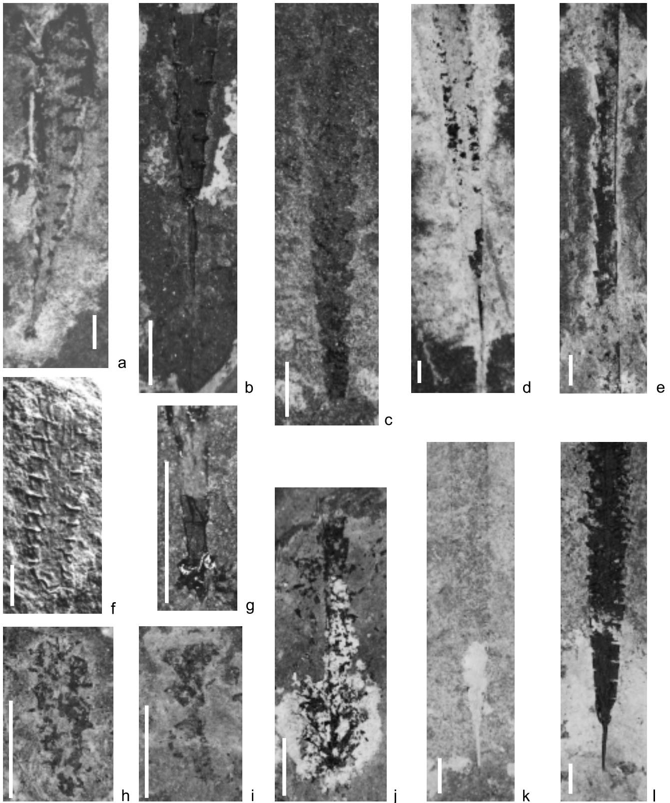
Fig. 8. a, g — Parakidograptus acuminatus (Nicholson), sample BS. 8: a — evolutionary younger, adult form with root-like virgellar structure, g — virgellar structure in detail; b — Normalograptus balticus (Pedersen), sample BS. 17, form with a stout virgella and thickened aperture rims; c — Glyptograptus ex gr. tamariscus , sample BS. 18; d — Normalograptus rectangularis (M'Coy), sample BS. 17; e — Atavograptus atavus (Jones), sample BS. 18; f — Cystograptus ancestralis Štorch, adult form, sample BS. 7; h — Paraclimacograptus innotatus (Nicholson), sample BS. 19; i — Dimorphograptus confertus (Nicholson), sample BS. 19, proximal part, the same specimen as on Figure 6i; j — Pseudorthograptus obtus (Rickards and Koren'), adult rhabdosome, sample BS. 19; k — Rhabdograptus toernquisti (Eles and Wood), reverse side with slightly undulating median septum, sample BS. 18; l — Neodiplograptus cf. elongatus Churkin and Carter, sample BS. 19; other explanations see Figure 4
