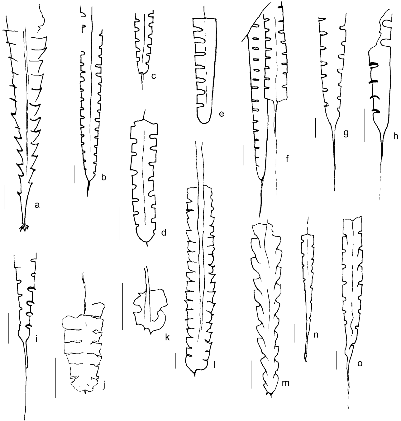
Fig. 5. a — Parakidograptus acuminatus (Nicholson), sample BS. 8, slightly curved form with root-like virgella; b, c — Normalograptus normalis (Lapworth), sample BS. 15; d, e — Normalograptus medius (Törnquist), sample BS. 16; f — Normalograptus rectangularis (M' Coy), sample BS. 22; g–i — Normalograptus balticus (Pedersen), sample BS. 17; g — flattened specimen, h, i — forms in half-relief with characteristically thickened aperture rims and very stout virgella; j–l — Cystograptus vesiculosus (Nicholson): j — sample BS.18, with only a few pairs of thecae, k — sample BS. 20, early astogenic stage, l — well preserved adult form with nematularium; m — Glyptograptus ex gr. tamariscus , sample BS. 18; n — Rhaphidograptus extenuatus (Elles and Wood), sample BS. 18, poorly preserved gracile rhabdosome; o — Rhaphidograptus toernquisti (Elles and Wood), sample BS. 18, reverse side with slightly undulating median septum; other explanations see Figure 4
