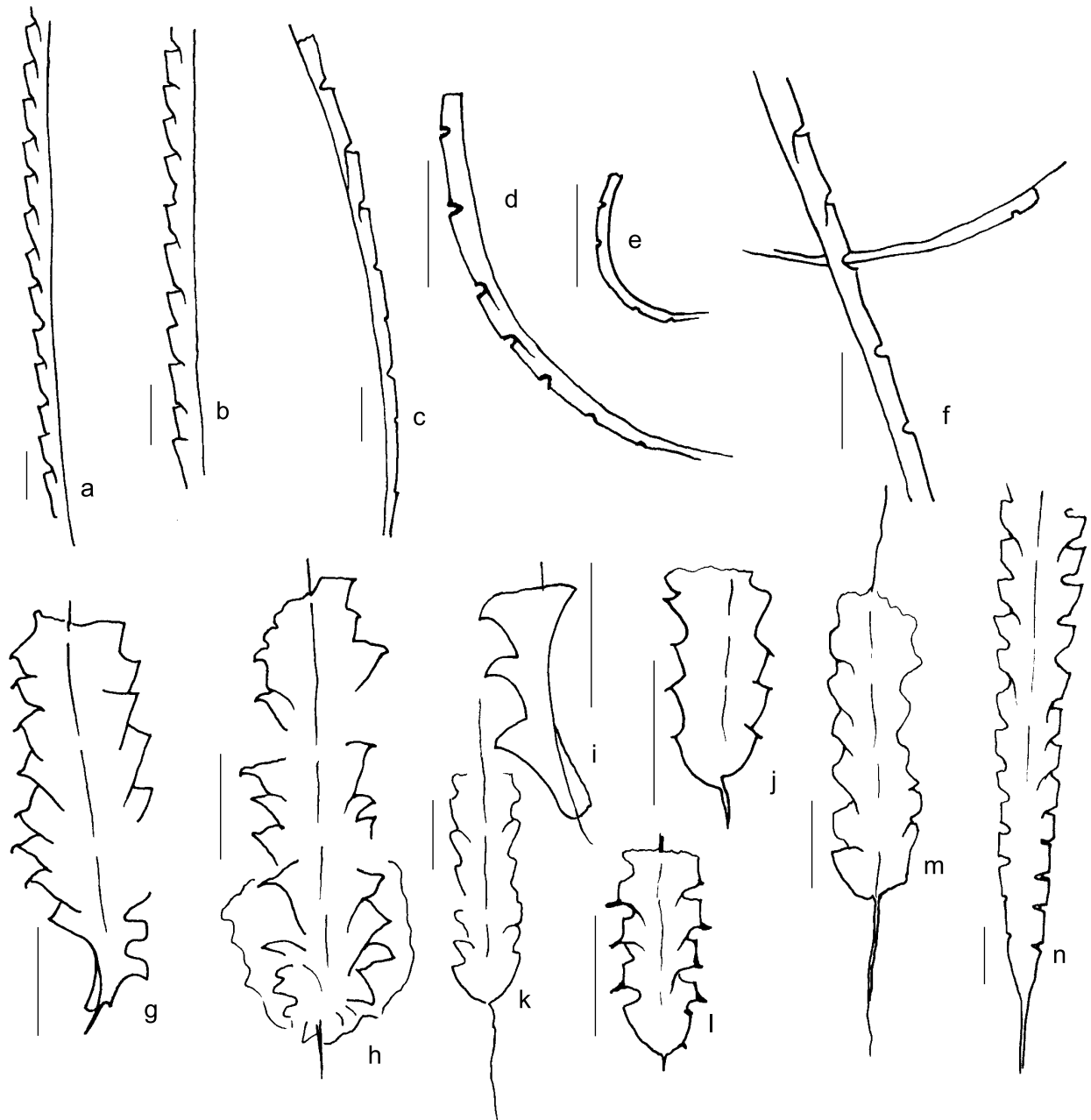
Fig. 6. a, b — Atavograptus atavus (Jones): a — sample BS. 18, b — sample BS. 19; c, f — Huttagraptus cf. praestrachani (Hutt and Rickards), sample BS. 18; d, e — Huttagraptus cf. incurvus Koren' and Bjerreskov, sample BS. 18; g — Dimorphograptus decussatus decussatus (Lapworth), sample BS. 19; h — Pseudorthograptus obuti (Rickards and Koren'), adult rhabdosome with preserved ?membranous tissue, sample BS. 19; i — Dimorphograptus confertus (Nicholson), proximal fragment, sample BS. 19; j — Sudburigraptus sp. 1, sample BS. 18; k, m — Diplograptus sp. 1, sample BS. 20; l — Paraclimacograptus innotatus (Nicholson), sample BS. 19; n — Neodiplograptus elongatus Churkin and Carter, sample BS. 19; other explanations see Figure 4
