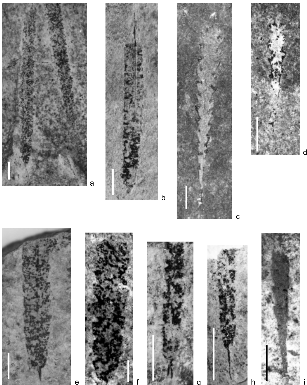
Fig. 7. a — Normalograptus cf. persculptus (Elles and Wood), sample BS. 4, left specimen is illustrated on Figure 4a; b — Normalograptus normalis (Lapworth), sample BS. Gr.; c — Parakidograptus acuminatus (Nicholson), sample BS. 5 (the same specimen as on Figure 4r); d — Parakidograptus primarius Li, sample BS. 8 (comp. Fig. 4k); e , f — Normalograptus parvulus (H. Lapworth), sample BS. 4; g — Normalograptus avitus (Davies), sample BS. Gr. (the same as on Figure 4h); h — Normalograptus miserabilis (Elles and Wood), sample BS. Gr.; i — Akidograptus ascensus Davies, sample BS. 7; other explanations see Figure 4
