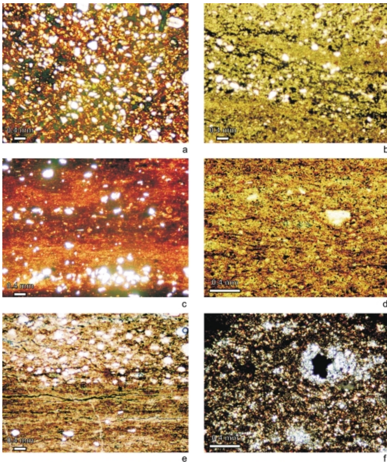
Fig. 2. a — silty-clayey very fine-grained and poorly sorted sandstone, sample BS. 2; b — silty to sandy claystone of beige and yellow-beige colour, with laminae enriched in coarser quartz grains, sample BS. 3; c — silty to sandy microlaminated beige-brown shale with the first graptolites, brown laminae are enriched with iron oxides, sample BS. 4; d — clayey shale with very sparse grains of quartz, sample BS. 5; e — transition between clayey shale (lower part) and black laminated chert (upper part), in clayey shale a few detrital quartz grains are visible, sample BS. 5; f — details of black laminated chert, white is chalcedony, black — framboids of pyrite, sample BS. 5
