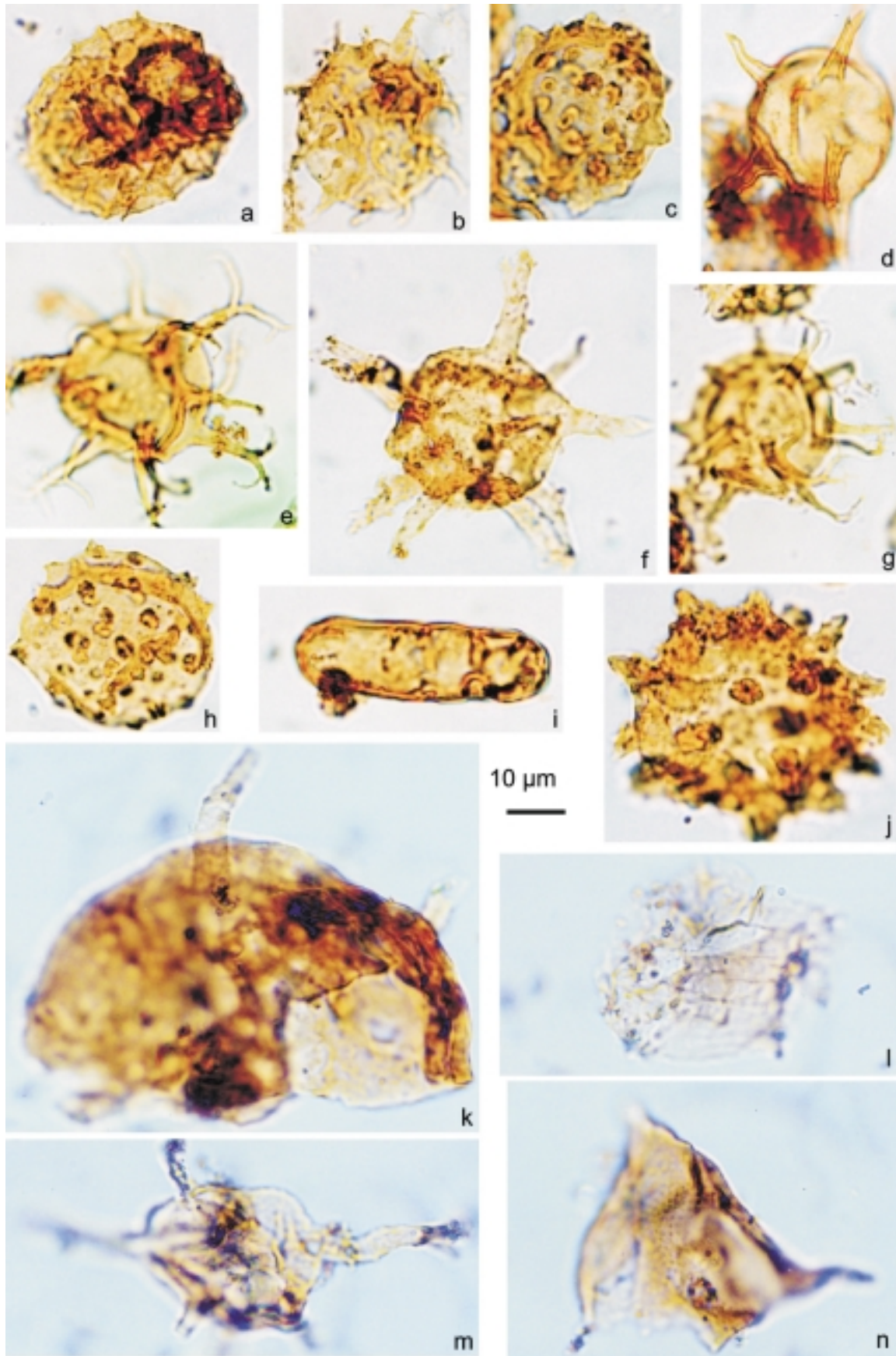
Fig. 10. Acritarchs from the Bardo Syncline
