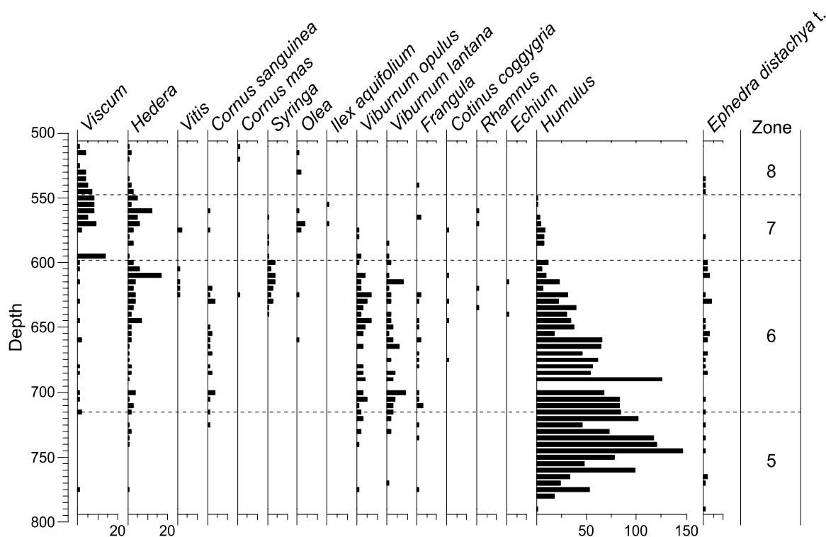
Fig. 4. Special pollen diagram from the part of the Dziewule section showing the total number of pollen grains of selected plants found in three slides
