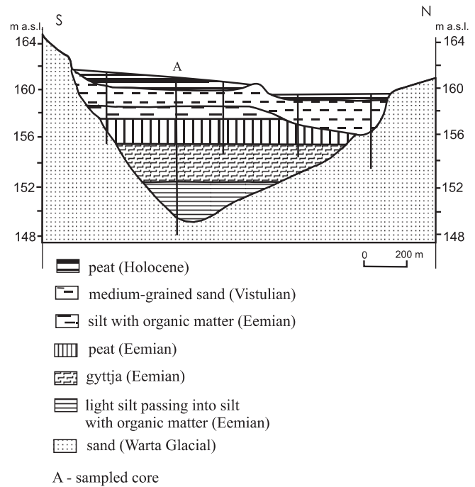
Fig. 2. Geological setting of the organogenic deposits at Dziewule
