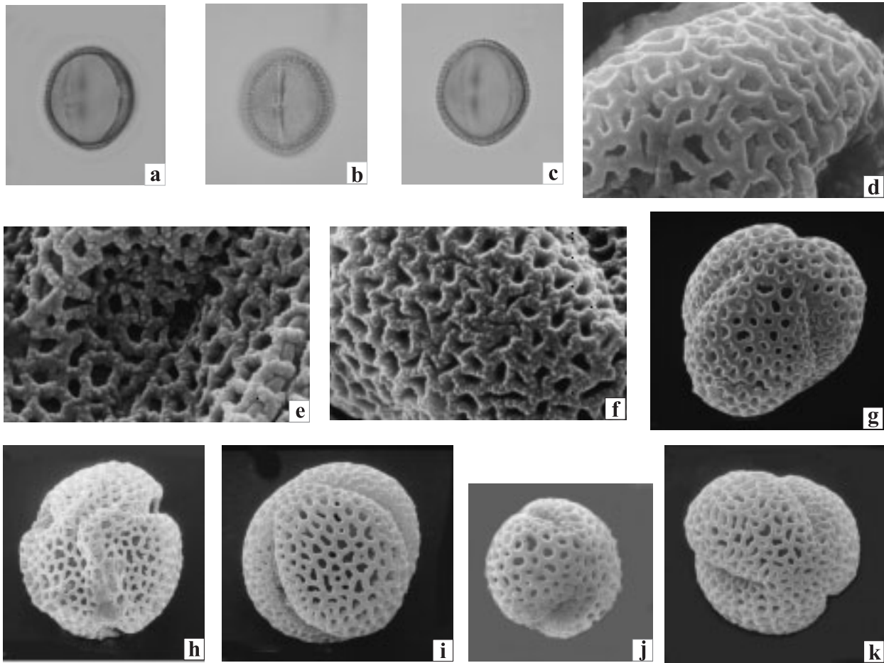
Fig. 5. Pollen grains of selected taxa from the Eemian at Dziewule against the Ferdynandovian, Mazovian and Brörup ones in Poland
