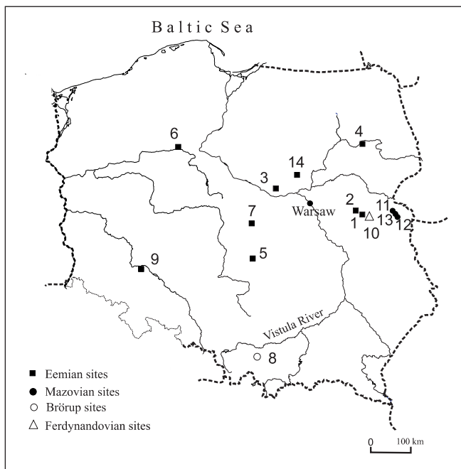
Fig. 1. Interglacial sites in Poland cited in the paper
