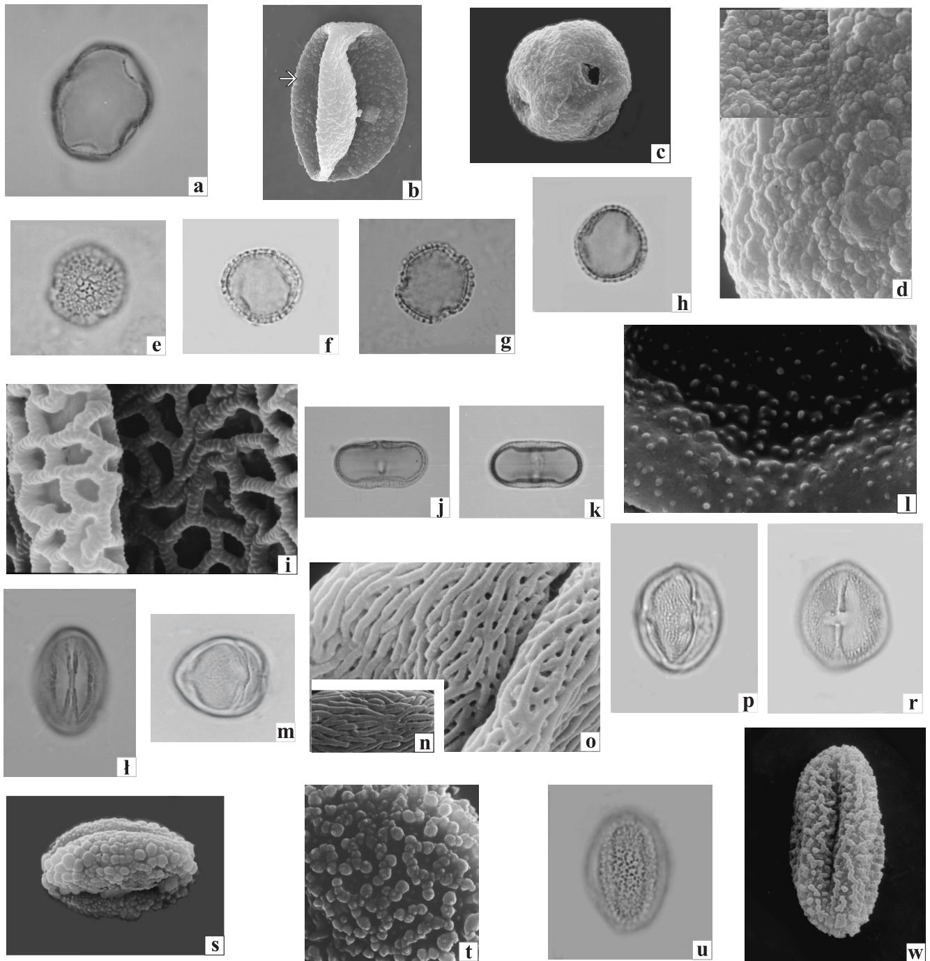
Fig. 6. Pollen grains of selected taxa from the Eemian at Dziewule against the Ferdynandovian, Mazovian and Brörup ones in Poland
