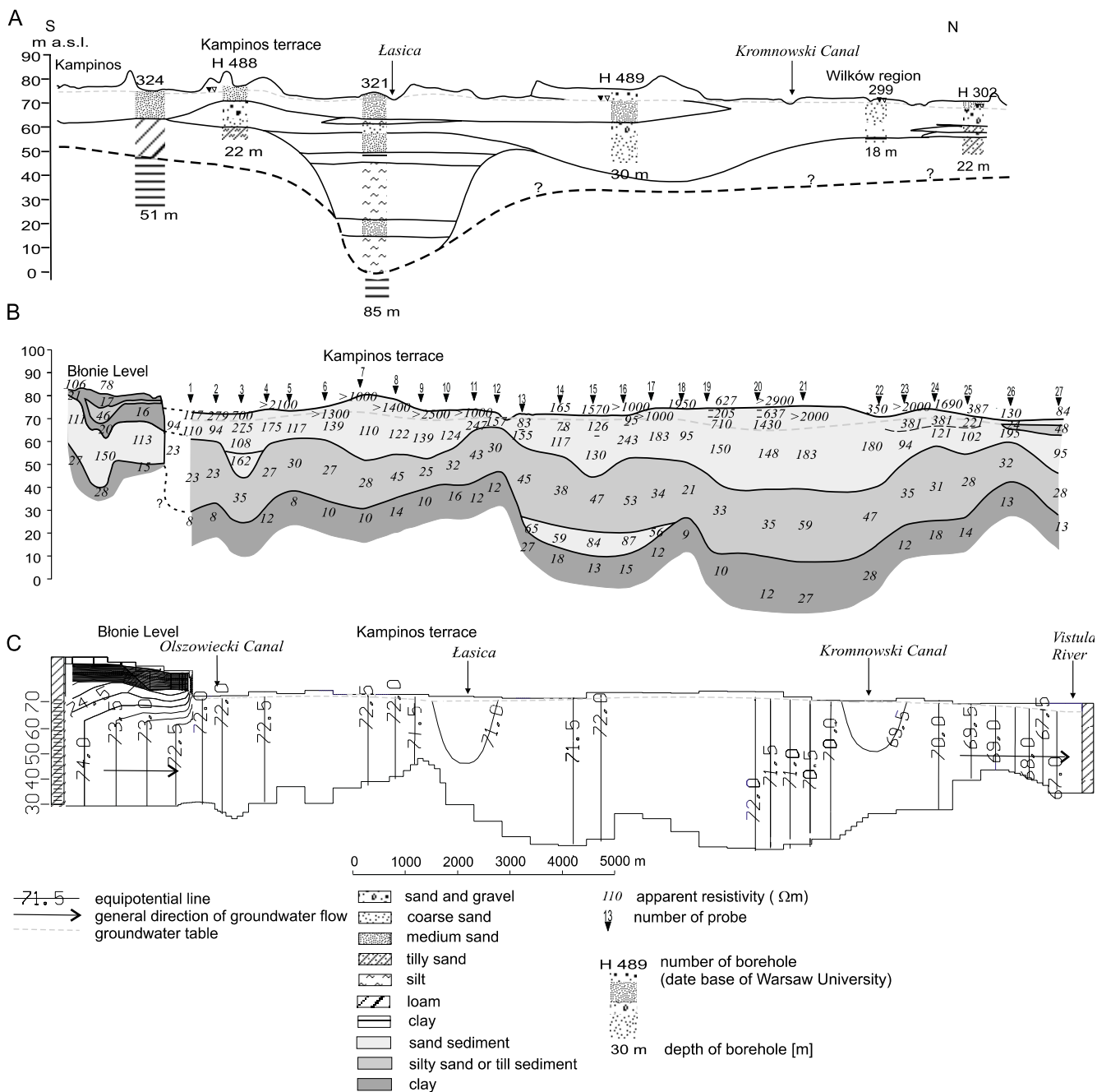
Fig. 2. A — geological cross-section, B — geophysical cross-section with geological interpretation, C — modelling cross-section
