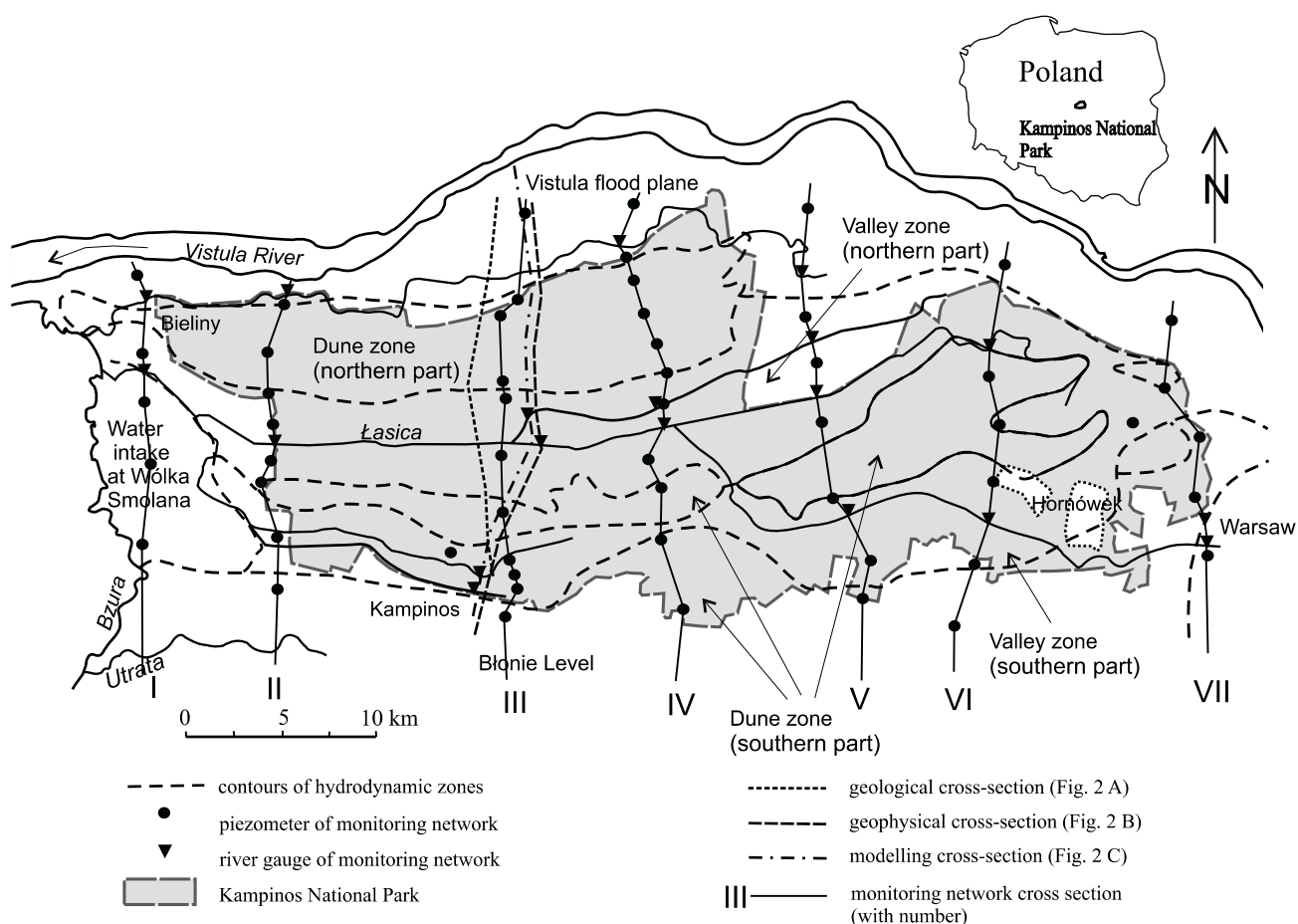
Fig. 1. Location of geological, geophysical and modelling cross-sections in the Kampinos National Park region
