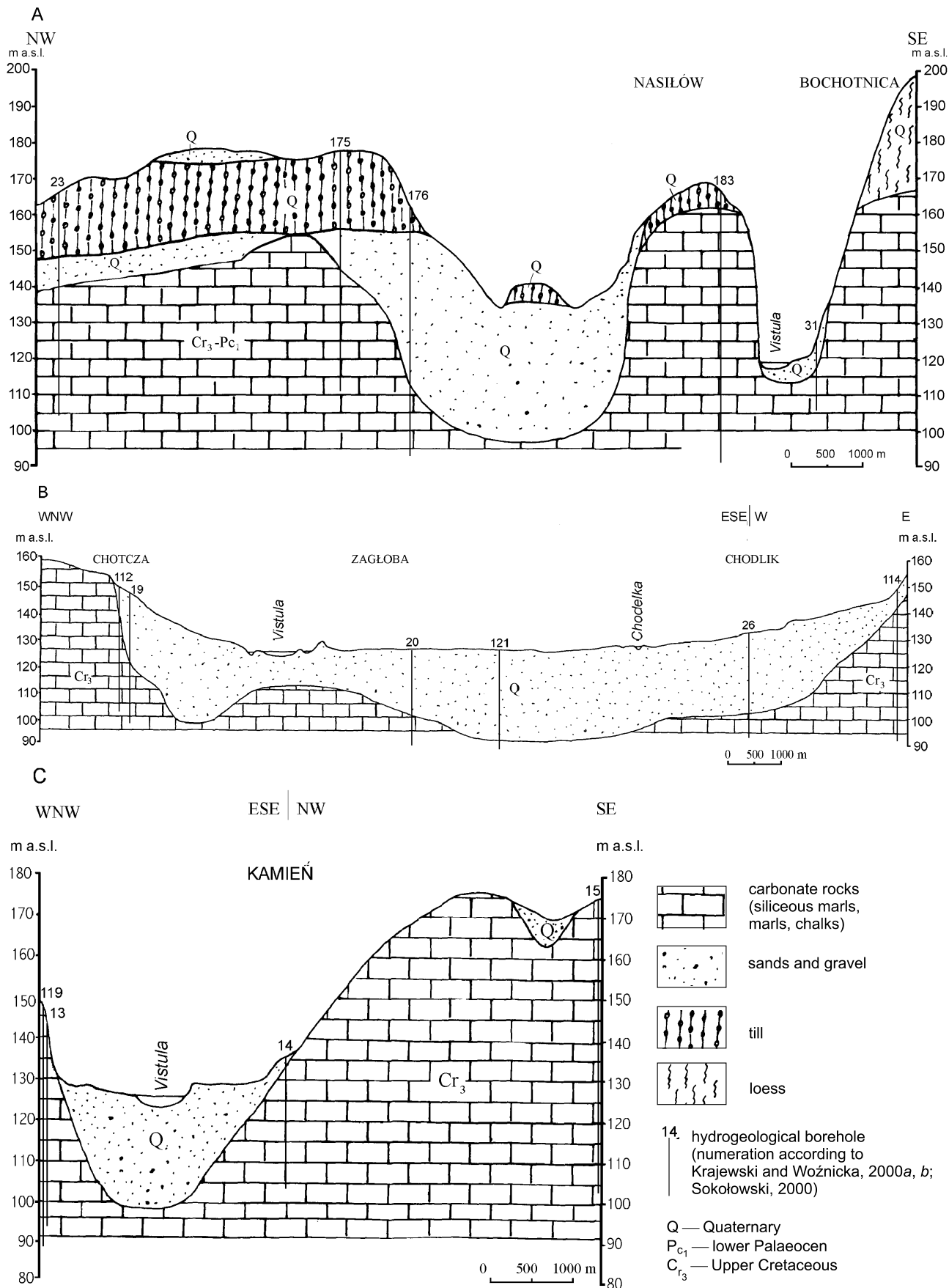
Fig. 2. Geological sections cutting the present and preglacial valleys of the Vistula
