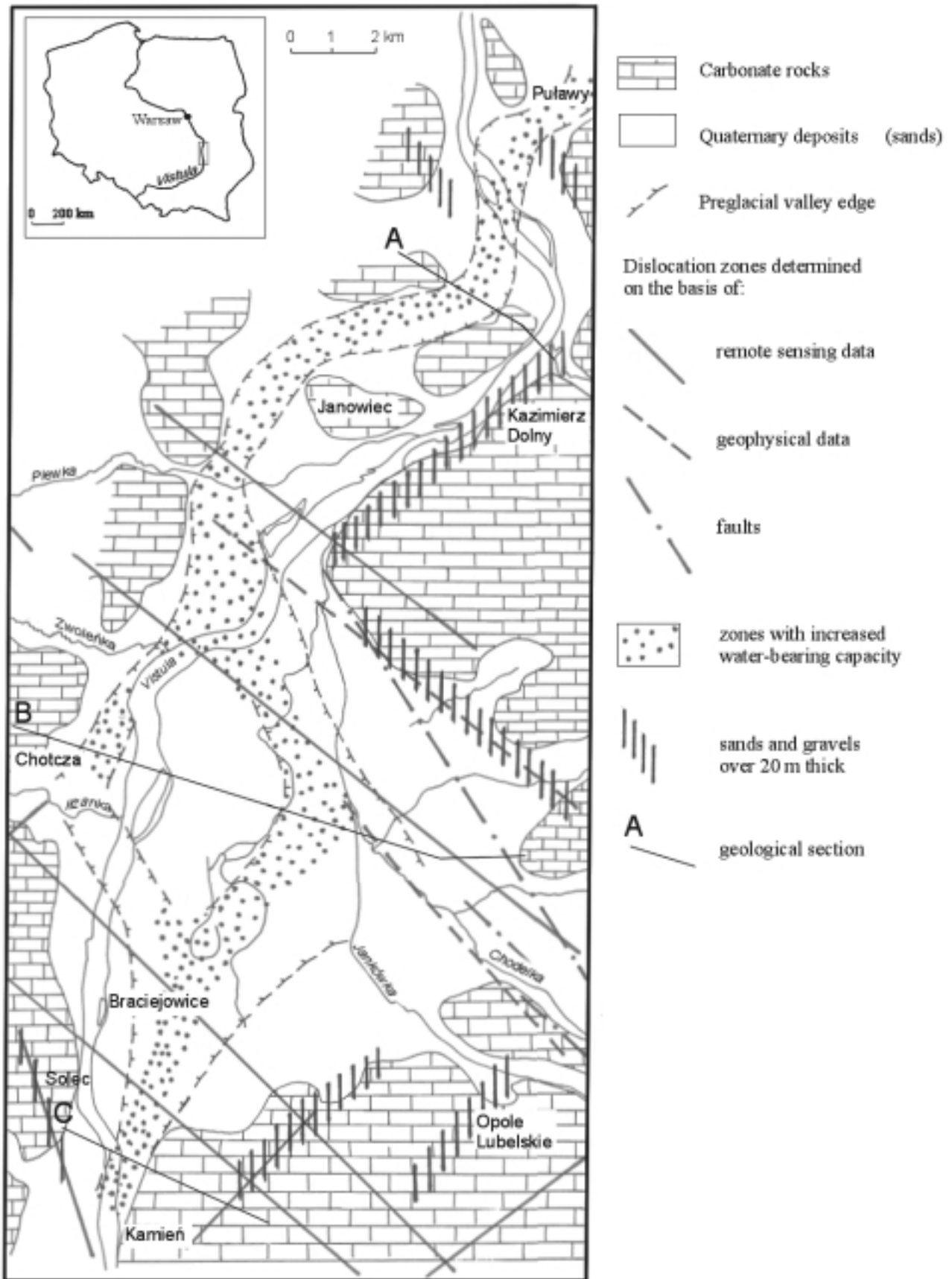
Fig. 1. Hydrogeological structure of the Vistula River valley versus dislocation zones
