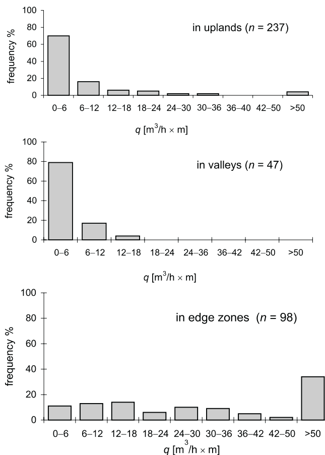
Fig. 3. Histograms of the distribution of specific discharges from wells according to location
