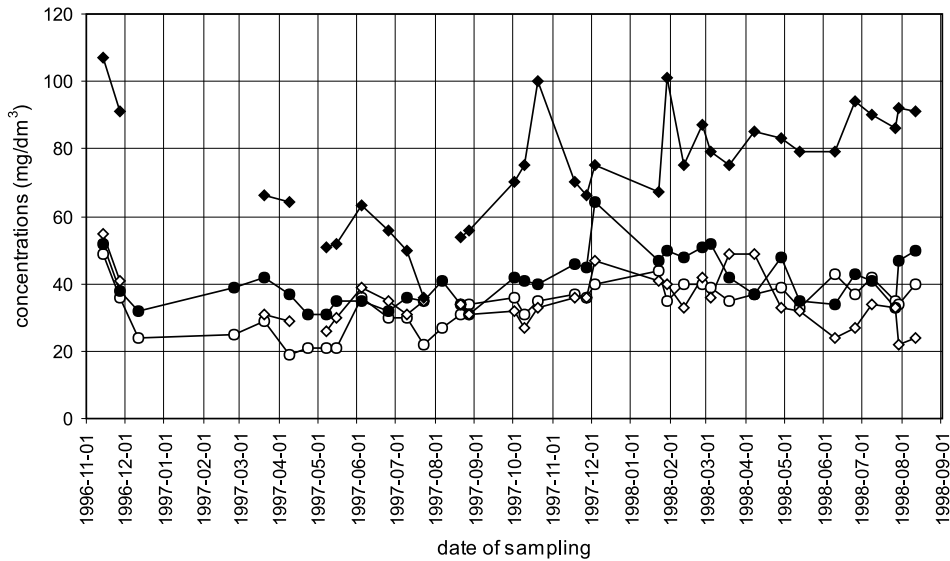
Fig. 5. Total nitrogen ( \text{mg/dm}^3 ) in inflow (black circles) and outflow (open circles) for wastewater after biological treatment (bed A); total nitrogen ( \text{mg/dm}^3 ) in inflow (black diamonds) and outflow (open diamonds) for wastewater after mechanical treatment (bed B)
