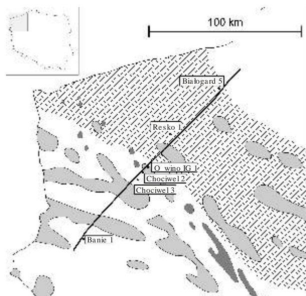
Fig. 2. Distribution of the salt structures in the Pomeranian segment of the Mid-Polish Trough
