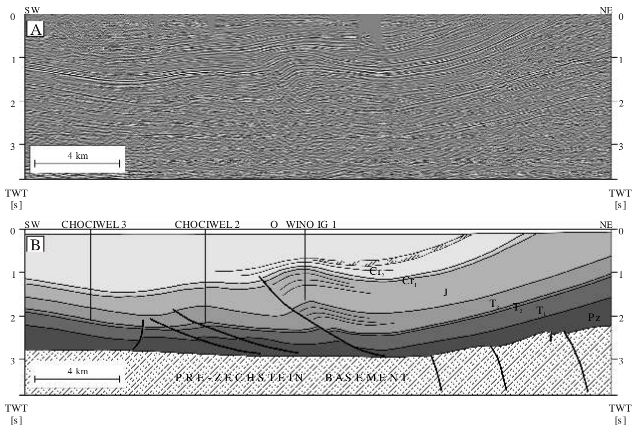
Fig. 4. Part of regional seismic profile from the Pomeranian segment of the Mid-Polish Trough showing details of the O wino compressional structure: A — uninterpreted, B — interpreted
