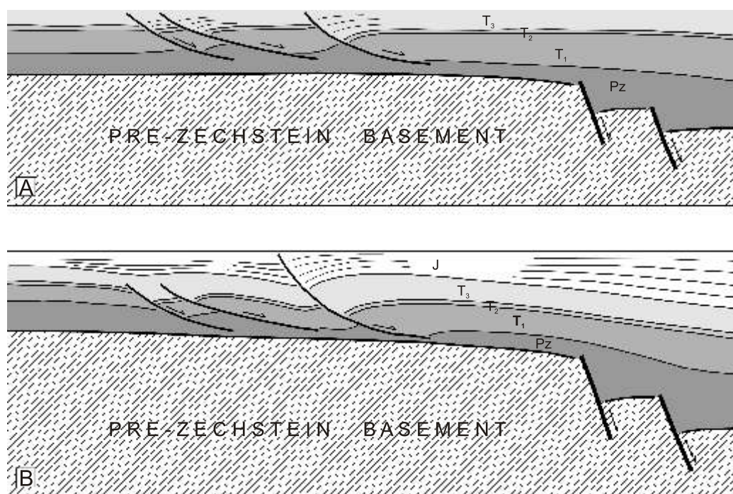
Fig. 5. Model of Late Triassic (A) and Late Jurassic (B) configuration of the O wino structure based on the seismic profile from Figure 4 flattened on top of Triassic and top of Jurassic respectively
