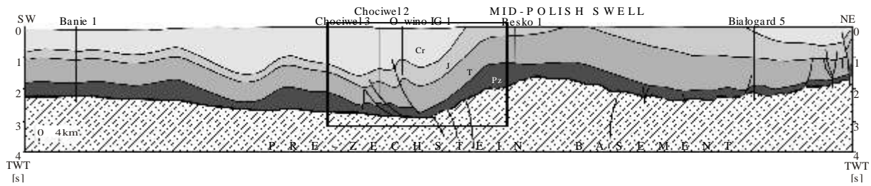
Fig. 3. Geological cross-section based on an interpreted regional seismic profile from the Pomeranian segment of the Mid-Polish Trough; location — see Fig. 1
