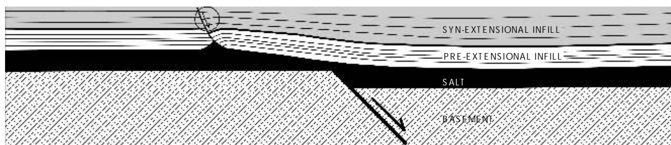
Fig. 1. Model of development of a listric normal fault within post-salt deposits due to decoupled faulting within the basement, based on results of analogue modelling (after Withjack and Calloway, 2000, modified); note local thickness increase of syn-extensional deposits above the hangingwall towards the listric fault (circle), and regional thickness increase of syn-extensional deposits towards basin centre
