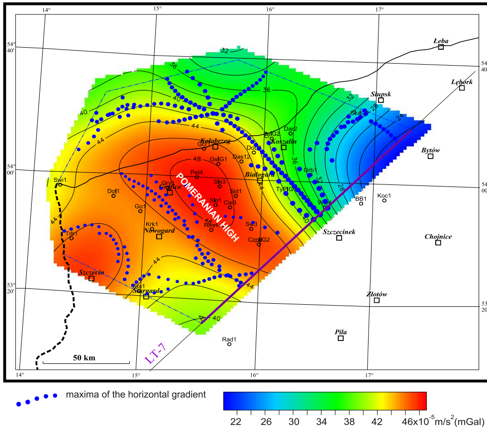
Fig. 4. Map of the “stripped” gravity anomalies continued upwards to 20 km
