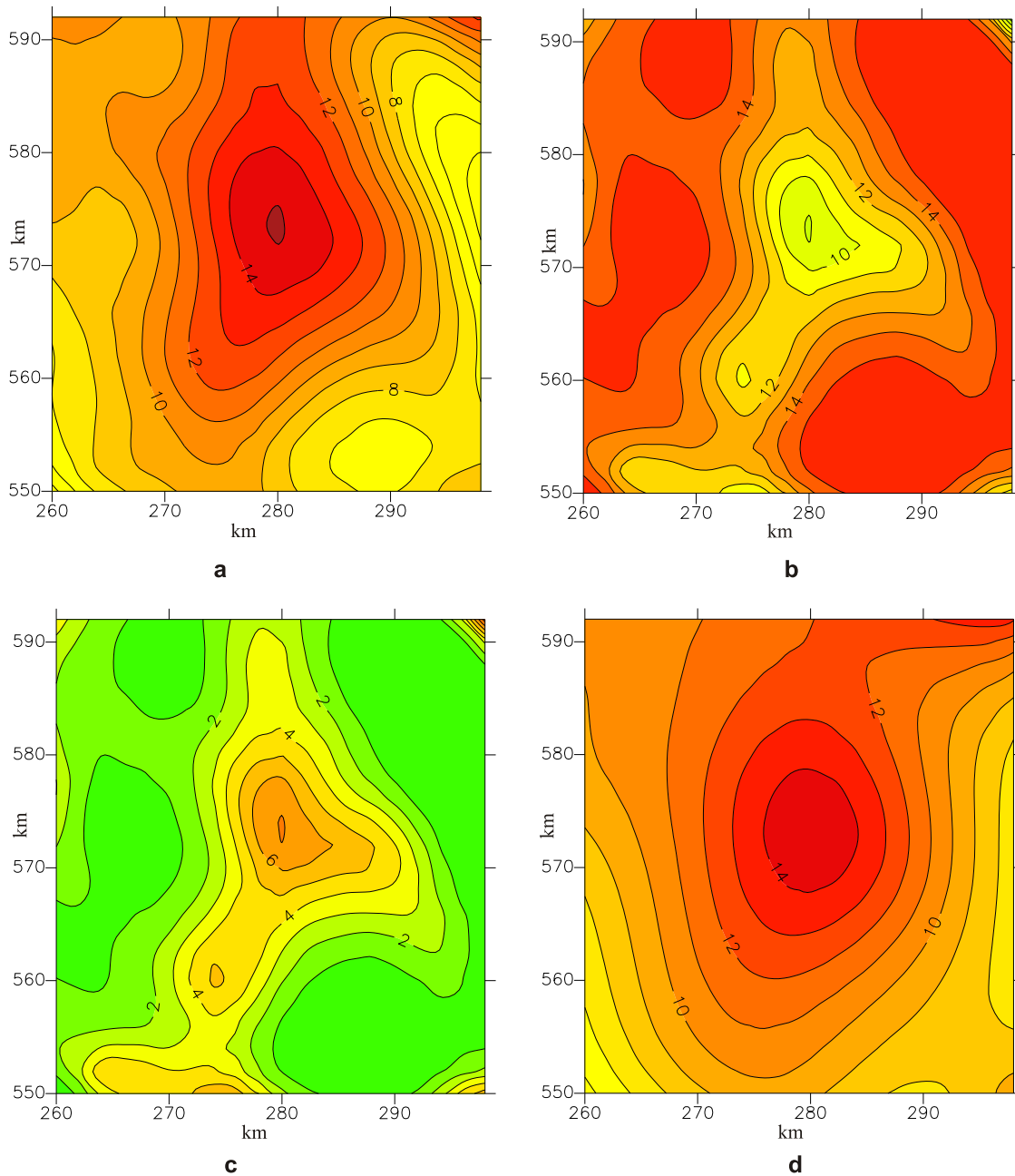
Fig. 6. 3D inversion of the “lepce” local “stripped” anomaly
