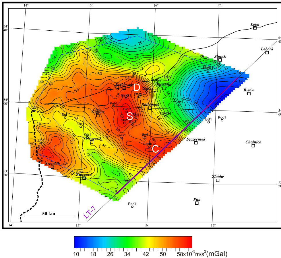
Fig. 3. Map of the "stripped" gravity anomalies caused by the sub-Zechstein basement
