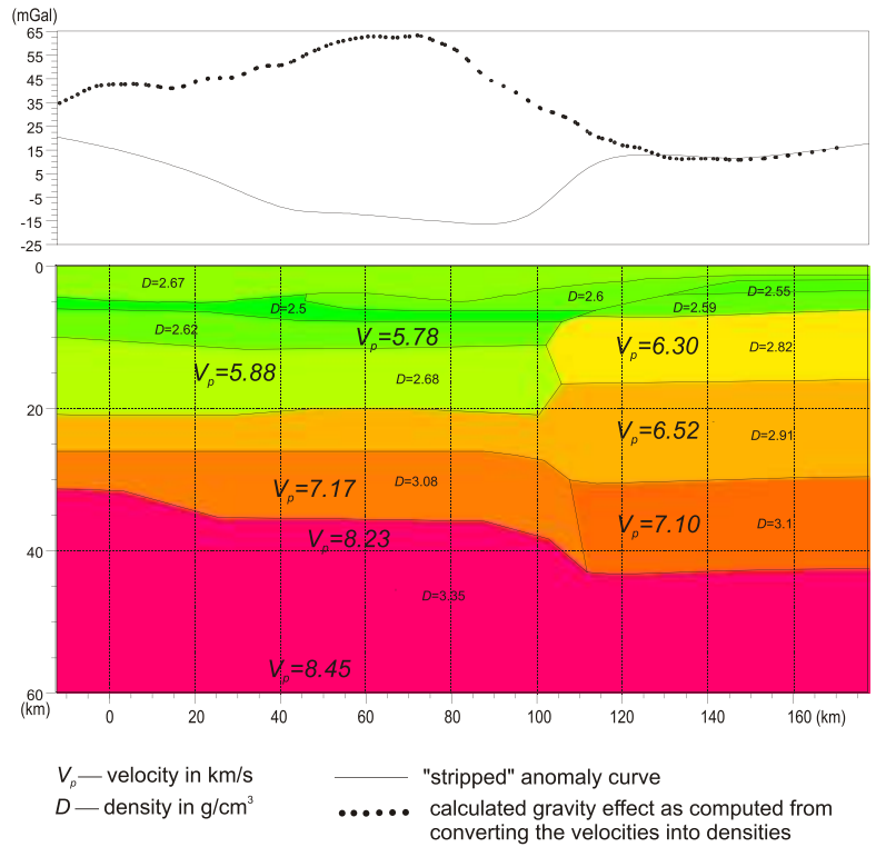
Fig. 7. P-wave velocity model of profile A (after Guterch et al. , 1994) (bottom) and the comparison between the calculated and "stripped" gravity anomalies along profile A (top)
