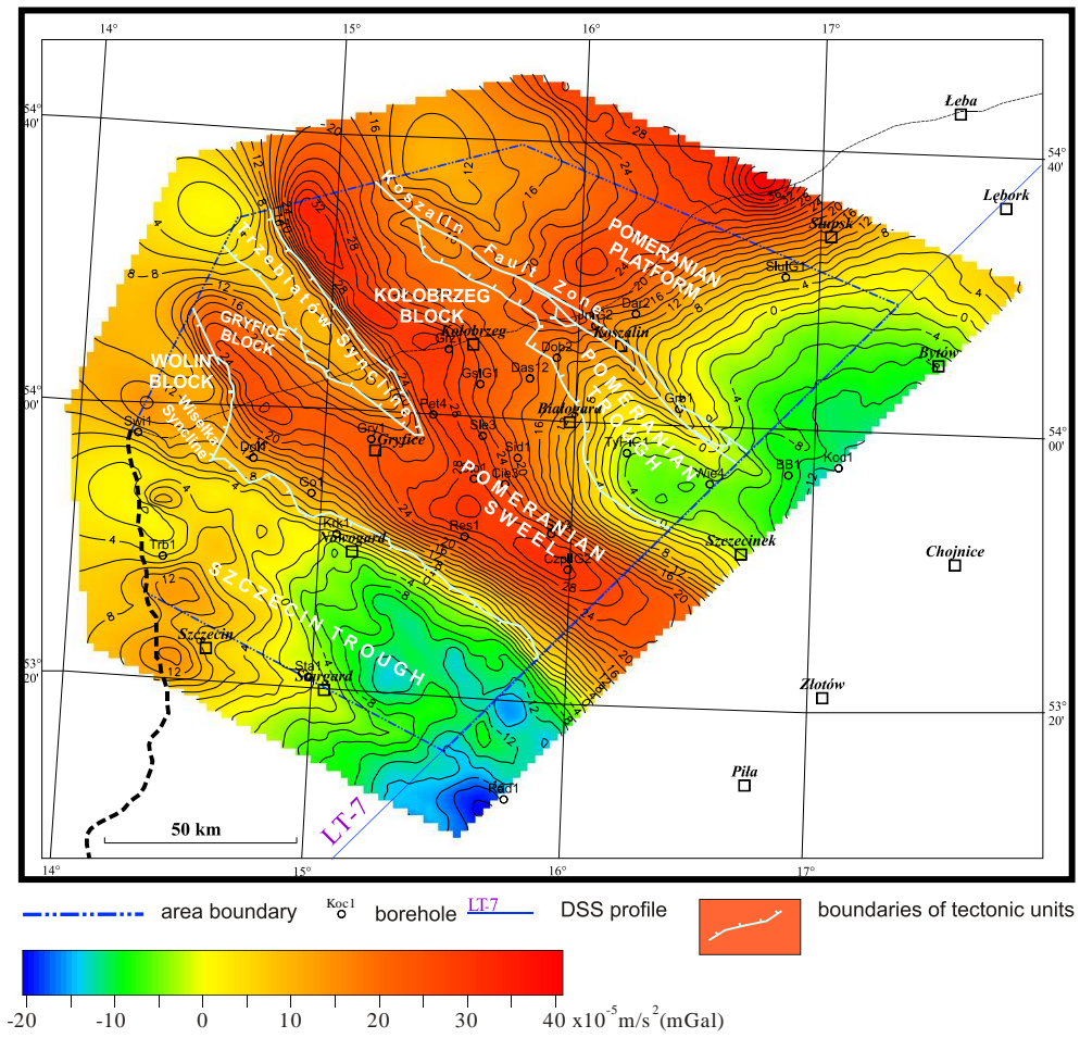
Fig. 2. Map of the Bouguer anomalies at the background of the main tectonic units
