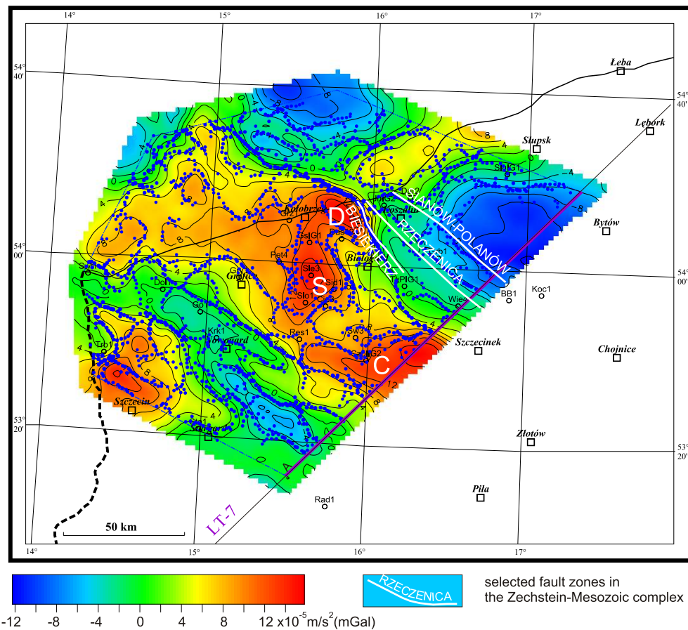
Fig. 5. Map of the local “stripped” gravity anomalies
