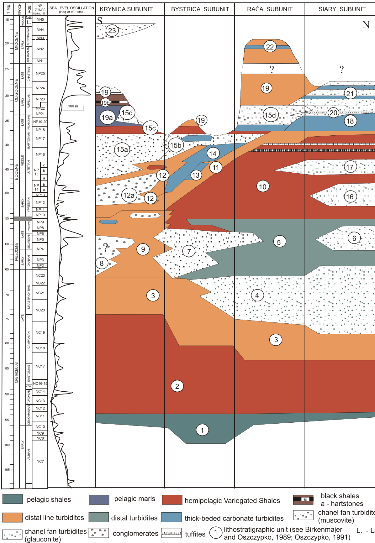
Fig. 2. Lithostratigraphy of the Magura Nappe in Poland (after Oszczytko et al. , 1999; changed)
