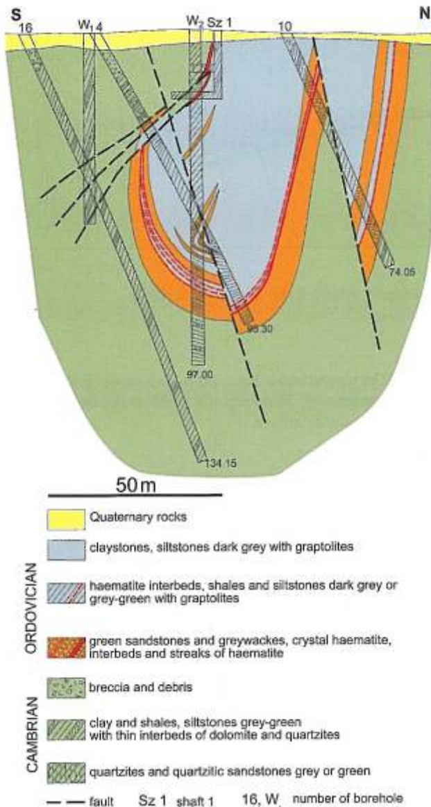
Fig. 3. Geological cross-section of Ordovician syncline along the boreholes 16, W 1 , 4, W 2 , 10 and shaft 1
