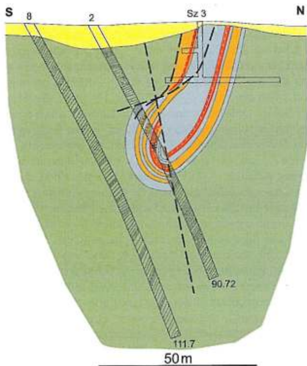
Fig. 5. Geological cross-section of Ordovician syncline along the borehole 8, 2, and shaft 3
