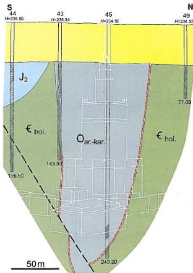
Fig. 9. Geological cross-section of Ordovician syncline along the boreholes 44, 43, 45 and 49; the depth of the syncline is shown by enclosed contour of the Palace of Culture and Science in Warsaw
