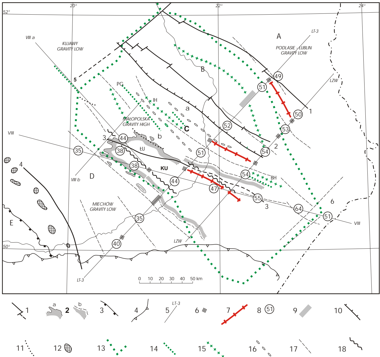
Fig. 1. Main geological units versus fundamental geophysical features
