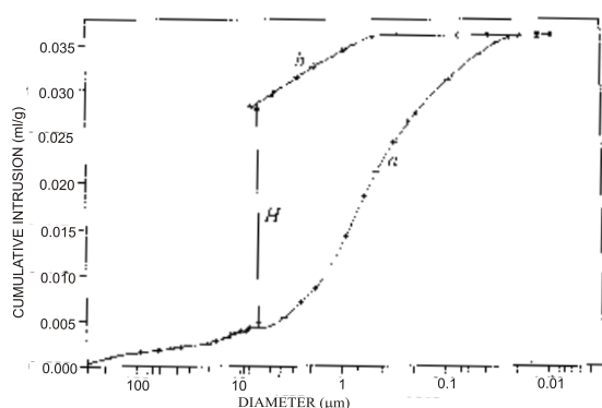
Fig. 3. Cumulative intrusion curve — obtained using the mercury capillary pressure method for the sample 7
