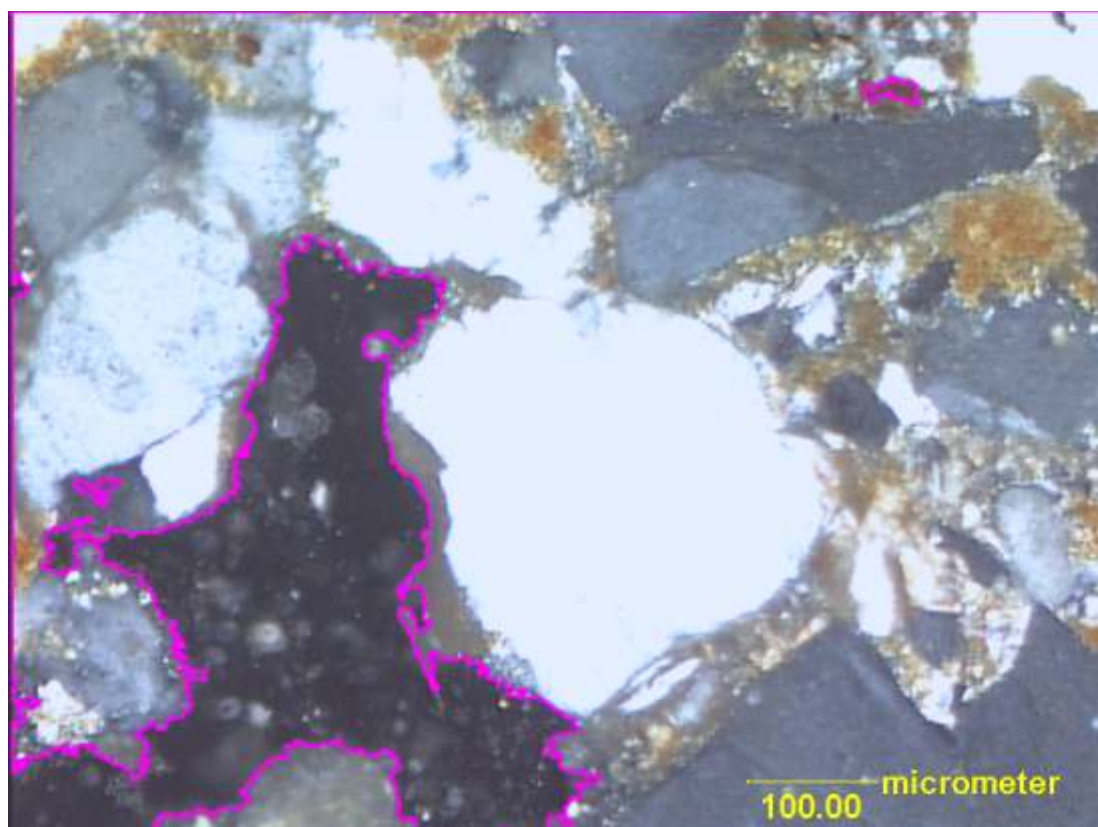
Fig. 1. Contoured pore area in sample 2 (magnification x 100)
