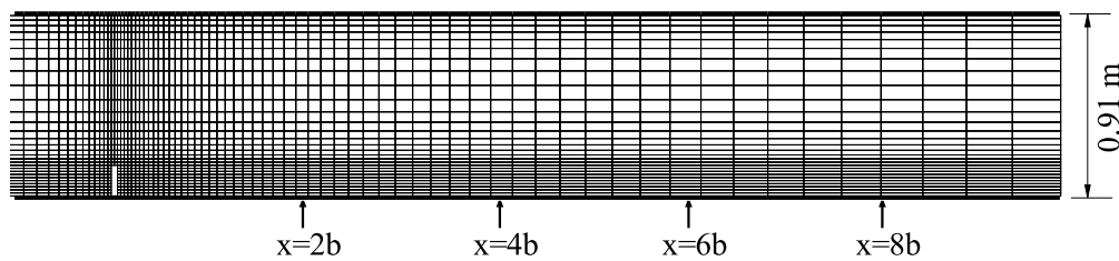
Fig. 1. Computational Mesh around a Spur-Dyke
