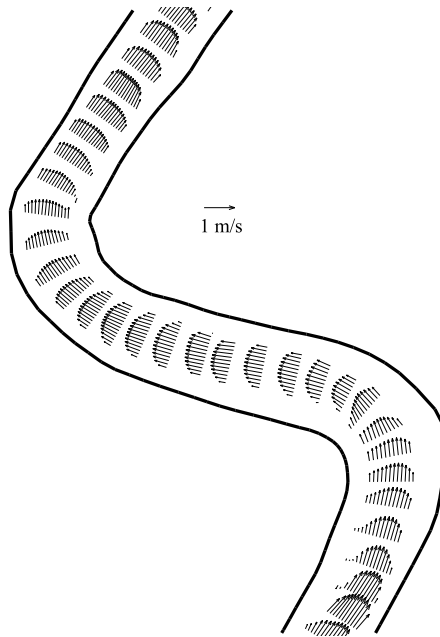
Fig. 13. Calculated Flow Field in part of the Dommel River (Standard k-\varepsilon Model)
