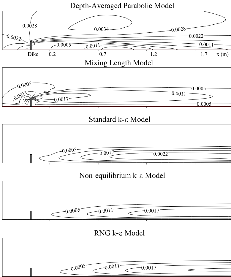
Fig. 4. Calculated Viscosities Velocities around a Spur-Dyke
