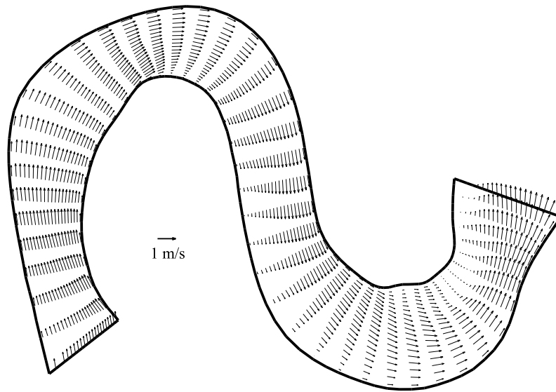
Fig. 9. Flow Field in the Fall River Calculated using the Standard k - \varepsilon Model
