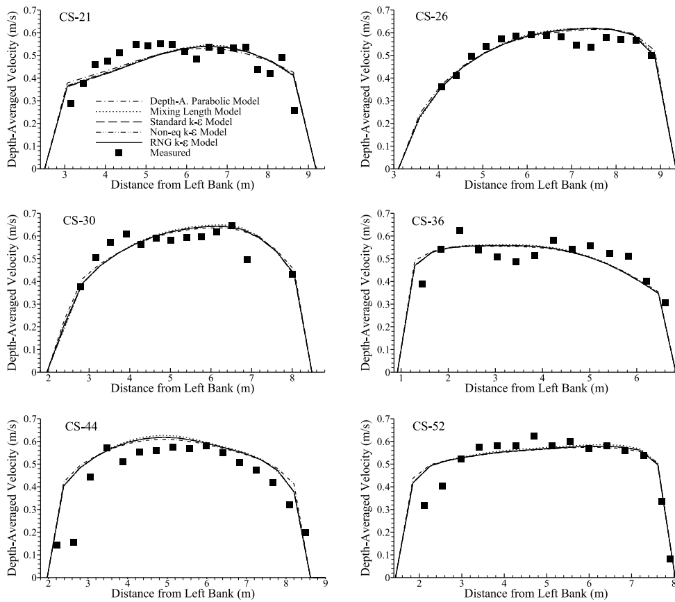
Fig. 14. Measured vs. Calculated Velocities in the Dommel River
