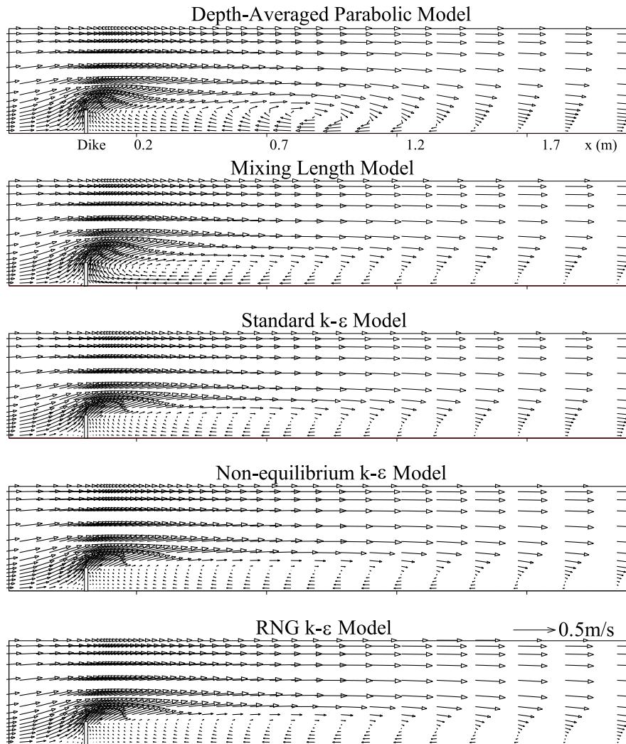
Fig. 2. Simulated Flow Patterns around a Spur-Dyke
