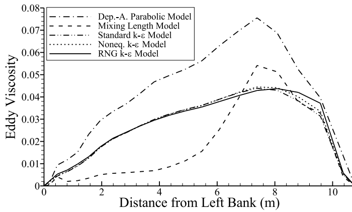
Fig. 10. Calculated Eddy Viscosities in CS-5A
