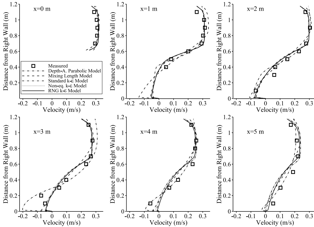
Fig. 6. Measured vs. Calculated Flow Velocities in the Sudden-Expanded Flume ( Q = 0.01815 \text{ m}^3/\text{s} )
