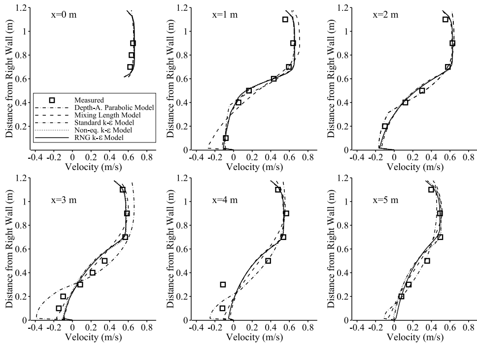
Fig. 7. Measured vs. Calculated Flow Velocities in the Sudden-Expanded Flume ( Q = 0.03854 \text{ m}^3/\text{s} )
