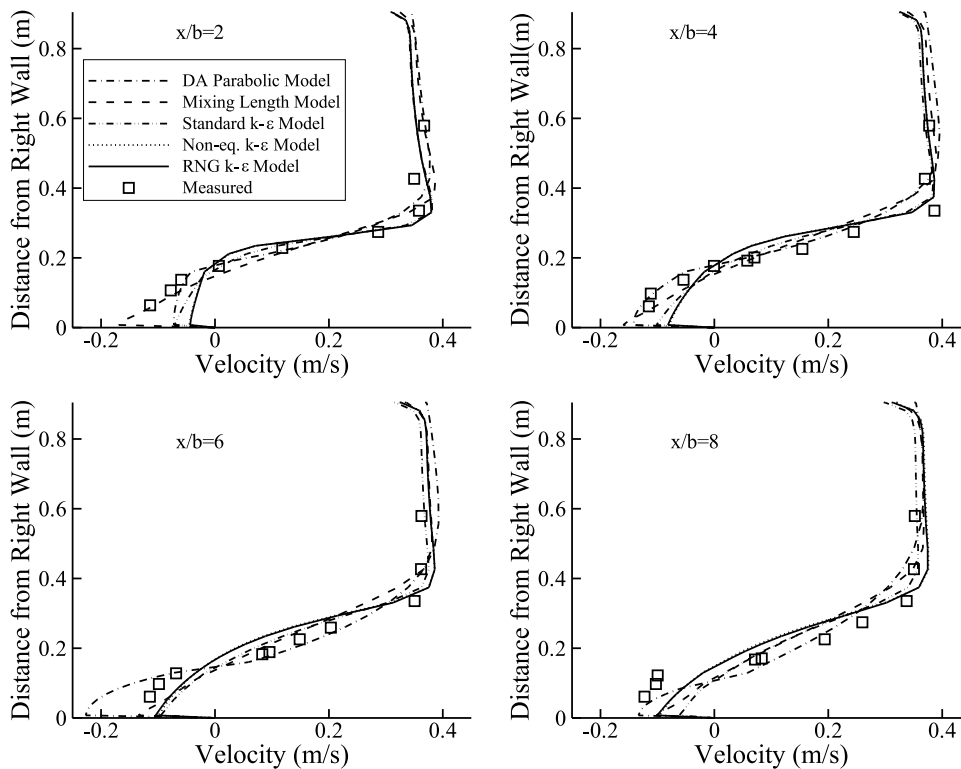
Fig. 3. Measured vs. Calculated Flow Velocities around a Spur-Dyke
