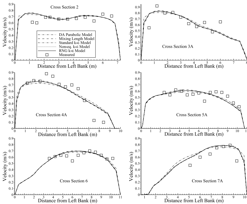
Fig. 11. Measured vs. Calculated Velocity in the Fall River
