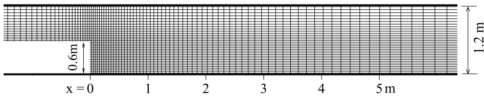
Fig. 5. Computational Mesh in the Sudden-Expanded Flume
