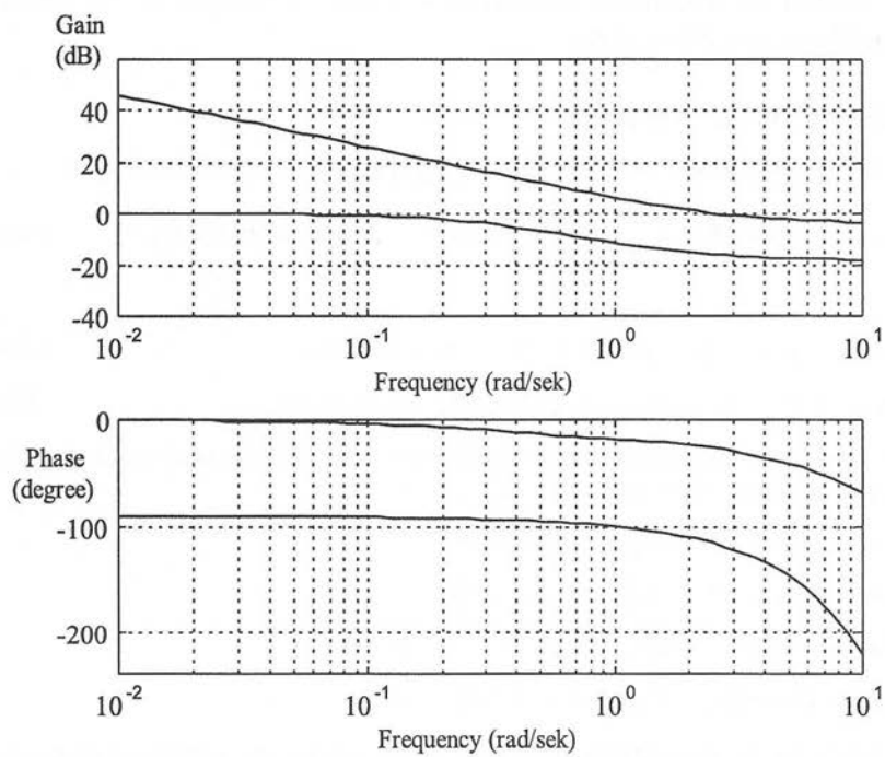
Figure 1. Bode magnitude and phase envelopes.
