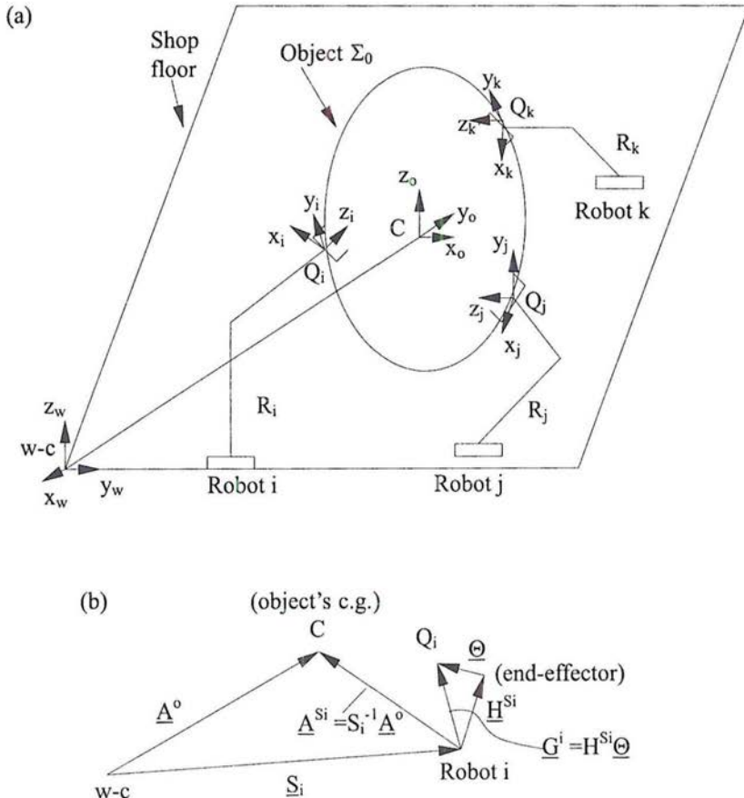
Figure 1. (a) An object handled by a system of m cooperating robots ( C = object's center of gravity, (x_0, y_0, z_0) = object coordinate frame, (x_i, y_i, z_i) = coordinate frame fixed to the i -th end effector). (b) Arrow diagram of the
