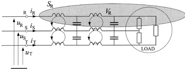
Fig. 6. Hypothetical space that confines phase R
