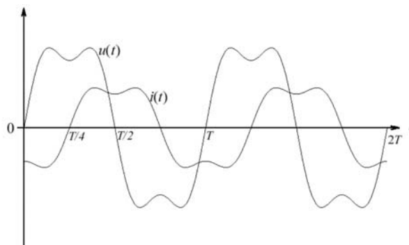
Fig. 6. Voltage and current in a circuit with non-zero distortion power,
