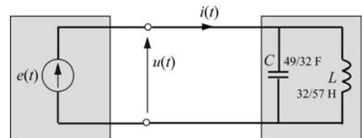
Fig. 3. Circuit with zero Budeanu's reactive power Q , but with energy
