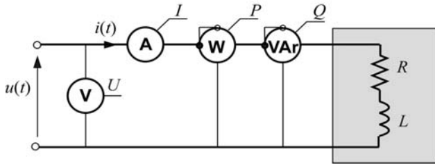
Fig. 1. Single-phase load with meters
