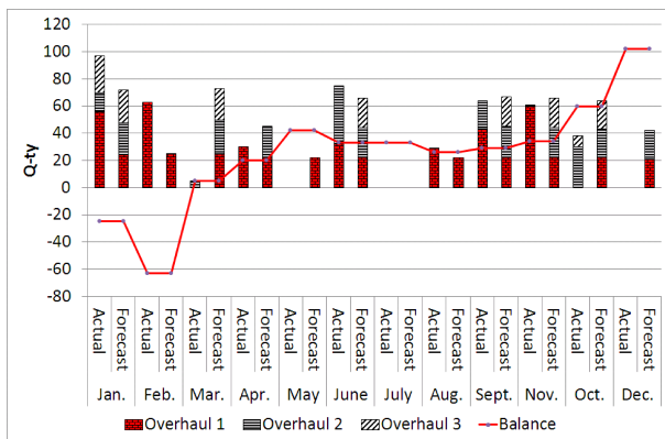
Fig. 4. Execution of forecast (moving average method) for spare compressor turbine blades first stage.
