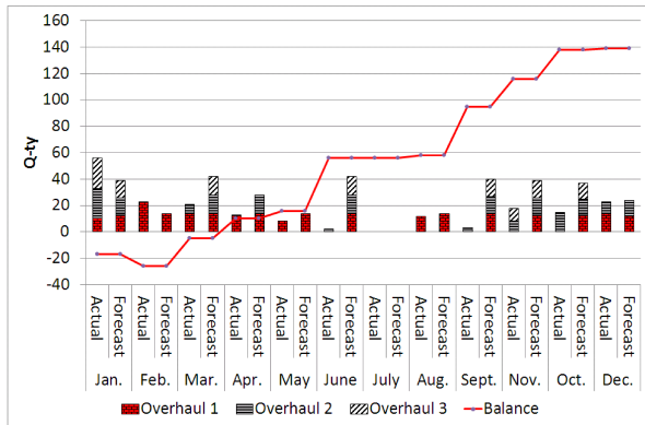
Fig. 2. Execution of forecast (moving average method) for spare compressor blades first stage.
