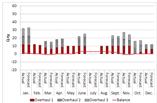
Fig. 7. Execution of forecast (ANN model) for spare bearing P/N 88.06.3276.
