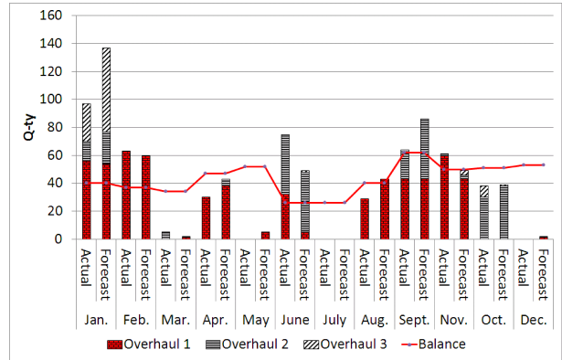
Fig. 5. Execution of forecast (ANN model) for spare compressor turbine blades first stage.
