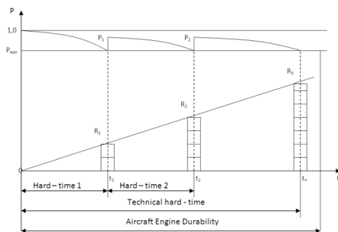
Fig. 1. Dependence of the probability(P) of work without failures and reliability (R) for hard – time operation of the aircraft engine.
