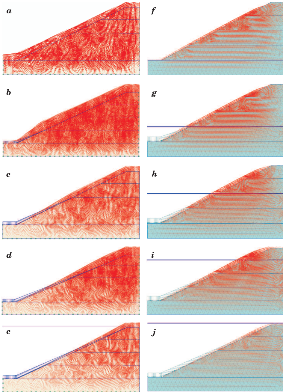
Fig. 2. Total displacements for the water level rising phase. A case of stepwise increase in water table a-e , displacements multiplied by 1,000. A case of linearly changing water flow f-j , displacements multiplied by 500
