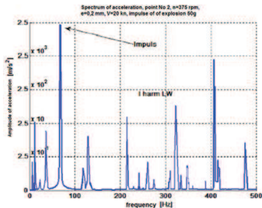
Fig. 14. The spectrum of acceleration with the inserted simulation of underwater explosion
