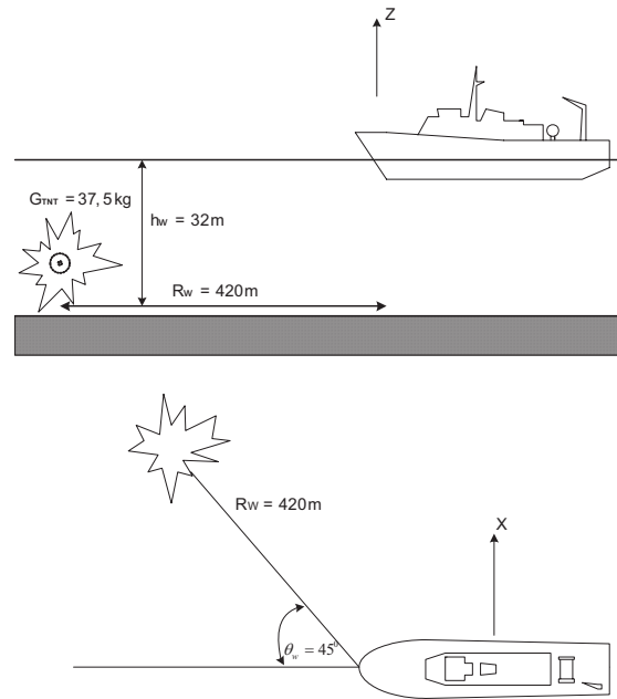
Fig. 3. Schematic diagram of the performed experimental test
