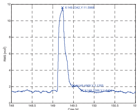
Fig. 6. Explosion, Starboard (PB), Intermediate bearing, Z axis
