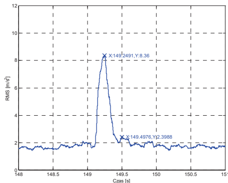
Fig. 5. Explosion, Port side (LB), Thrust bearing, X axis
