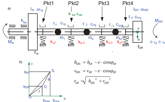
Fig. 12. Scheme of shaft line of minehunter where:
