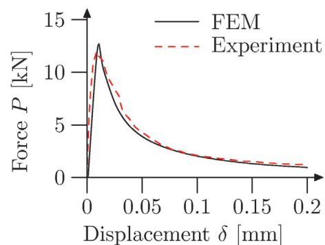
Fig. 7. Calculated contour map of parameter \kappa and force-displacement curve at shear force P_s = 10 kN using damage mechanics with Eqn. (6)
