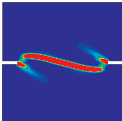
Fig. 13. Calculated contour map of parameter \kappa and force-displacement curve at shear force P_s = 10 kN using damage mechanics with Eqn. (10)
