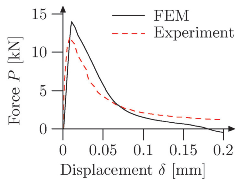
Fig. 13. Calculated contour map of parameter \kappa and force-displacement curve at shear force P_s = 10 kN using damage mechanics with Eqn. (10)
