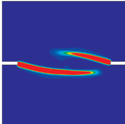
Fig. 12. Calculated contour map of parameter \kappa and the force-displacement curve at shear force P_s = 5 kN using damage mechanics with Eqn. (10)
