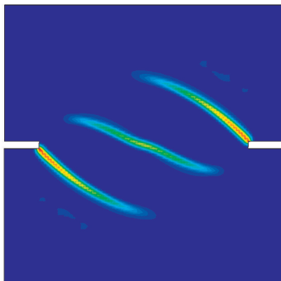
Fig. 14. Calculated contour map of parameter \kappa and force-displacement curve at shear force P_s = 38.5 kN using damage mechanics with Eqn. (10)
