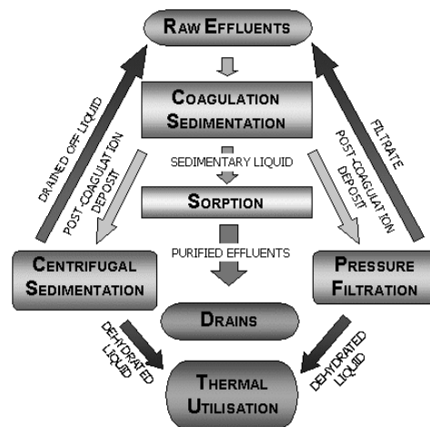
Fig. 1 Block diagram of effluent purification and post-production waste utilization at the timber processing plant [18]
