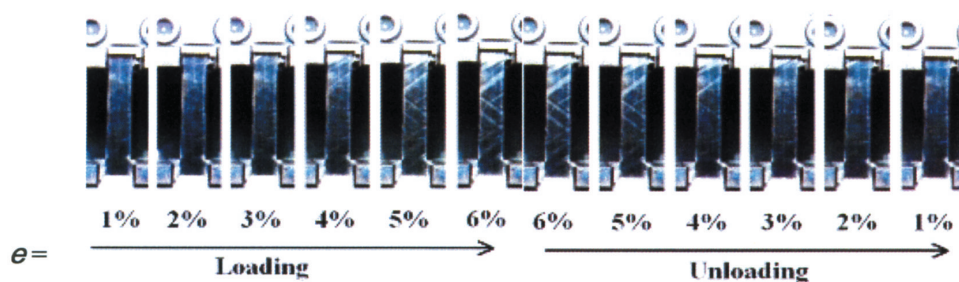
Fig. 6. Deformation patterns on TiNi SMA specimen surface due to phase transformations in tension test under strain rate = 1.6 \times 10^{-2} \text{ s}^{-1}
