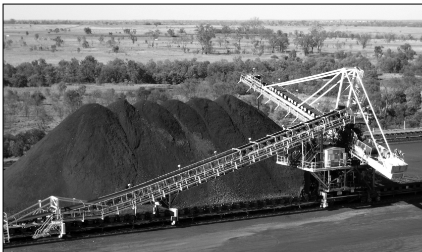
Fig. 3. Krupp coal stacker featuring tripper conveyor and non-slewing, luffing boom at RTCA Kestrel Mine [4]
