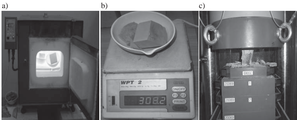
Fig. 1. Laboratory tests
