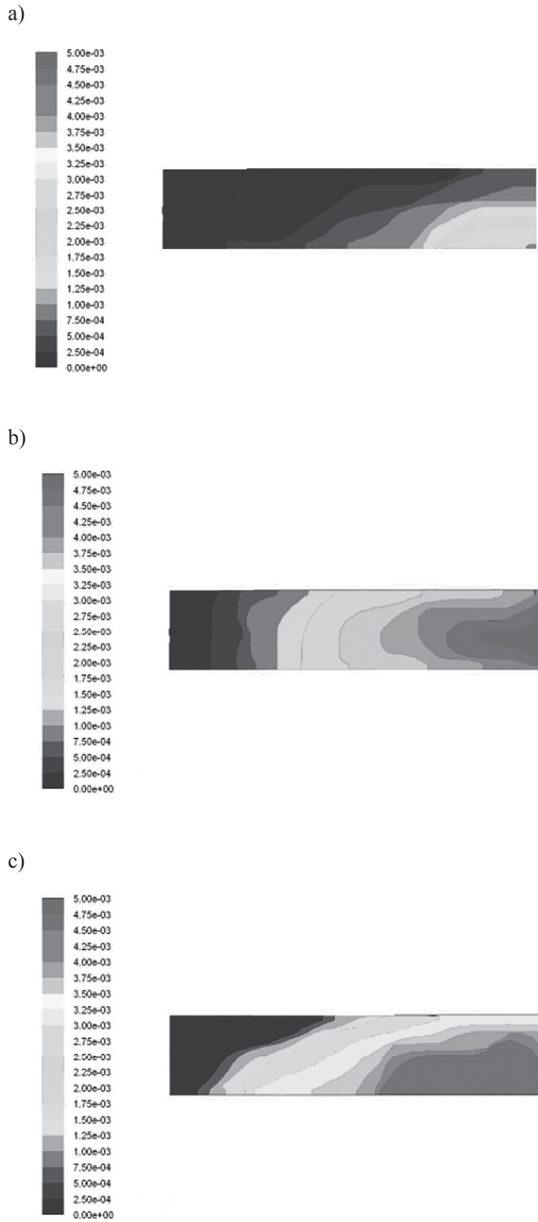
Fig. 3. Dust concentrations at several cross sections along Y direction: a) y = 0 ; b) y = 1.8 m; c) y = 3.5 m
