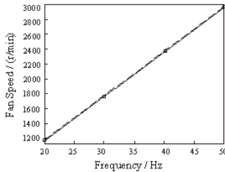
Fig. 5. Comparison of the second impeller acquired by two measuring methods: - - Measured curve by infrared speedometer; — Measured curve by tip pressure; ◻ Measured value by tip pressure
