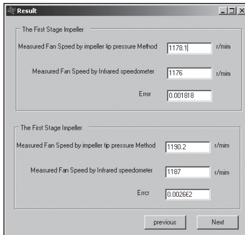
Fig. 3. The dialogue diagram of result
