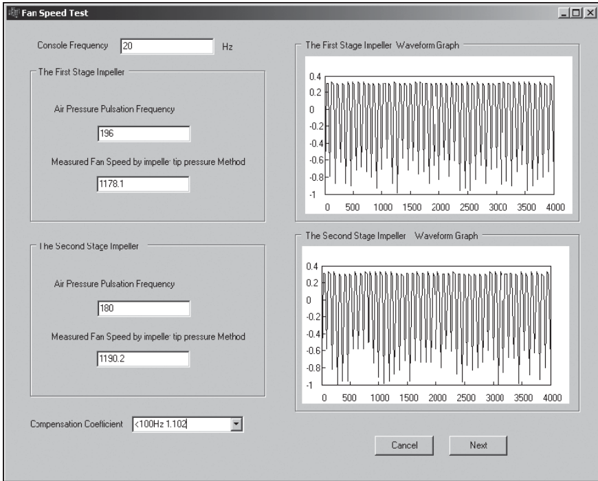
Fig. 2. The dialogue diagram of fan speed test
