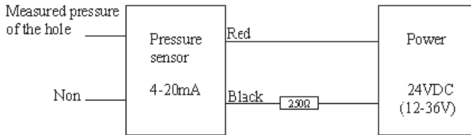
Fig. 1. Pressure sensor signal connection diagram
