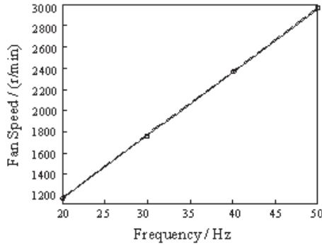
Fig. 4. Comparison of the first impeller acquired by two measuring methods
