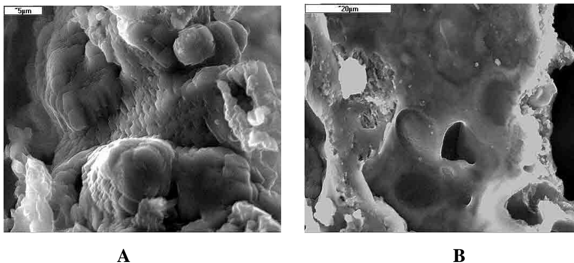
Photo 11 Sample 8 - the material from fireplace. A – secondary crystallized dolomite (See EDS – fig. 5 A). B – fragment of porous Si glass (see EDS fig. 5 B). SEM, magnification on scale.
