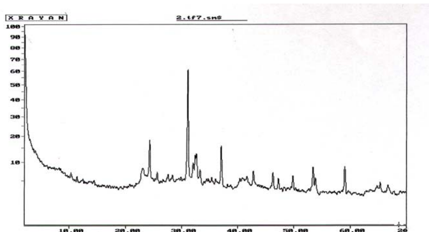
Fig. 4 X-ray pattern of burnt powder mixed with quartz, feldspars, carbonates and burned organic substance
