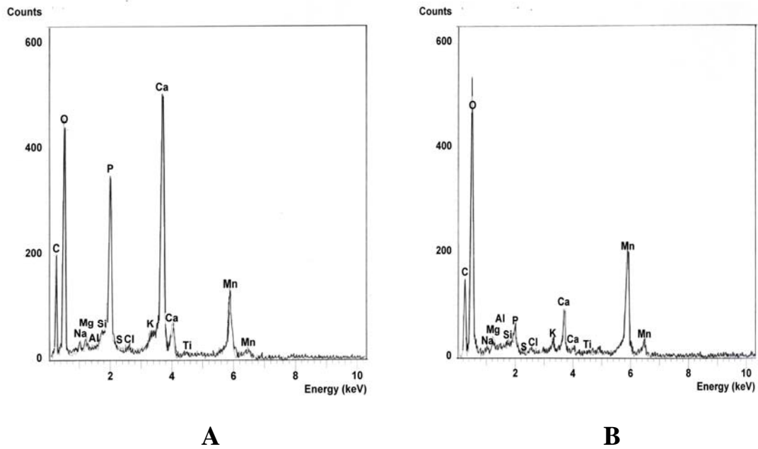
Fig. 7 EDS of sample no 10. Black organic substance coating alabaster vessels containing calcium phosphates (A) and Mn-oxides (B).
