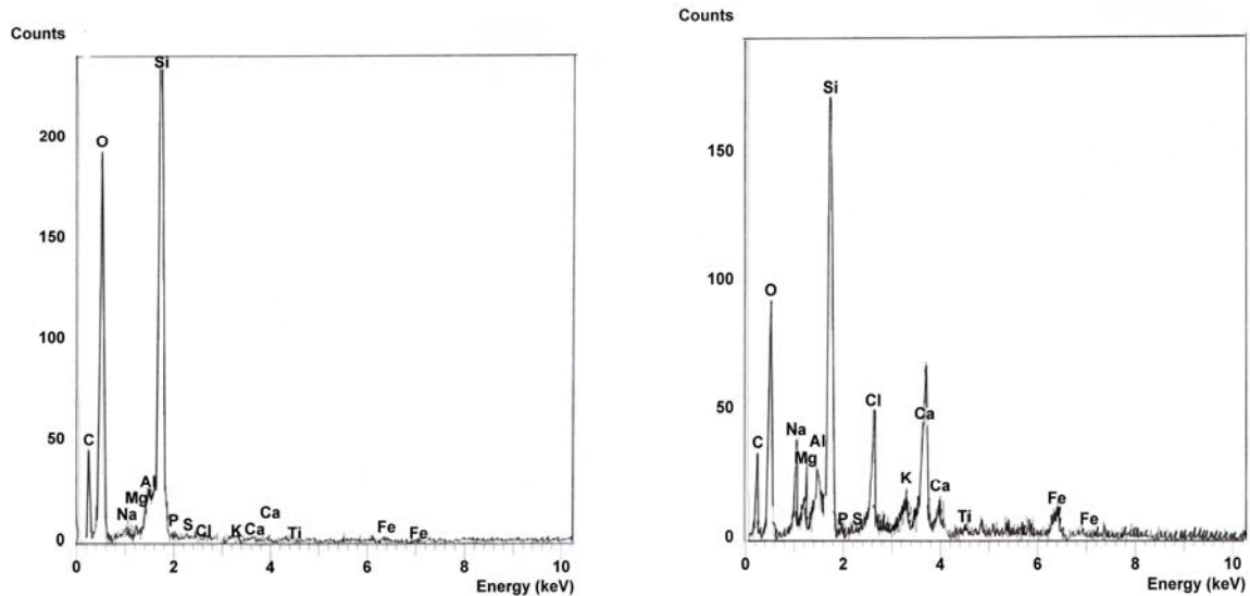
Fig. 6 EDS of sample no 9 - mineralized mat
