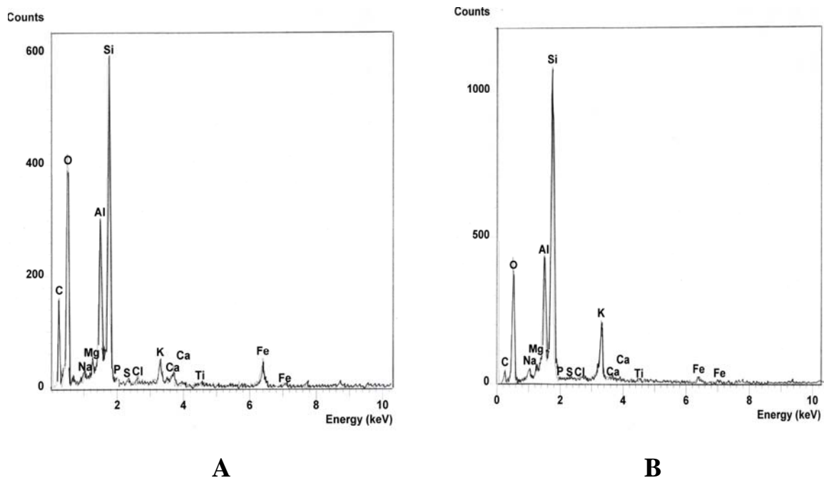
Fig. 3 EDS of sample no 5 – burnt grains of plant. One can see energetic peaks of Al, Si, C, K and Fe documenting presence of secondary mineralization as burnt organic matter.
