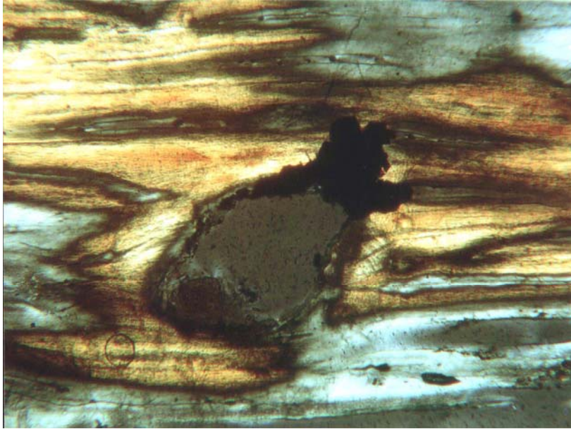
Photo 7. Alternation of cortical bone into secondary carbonates as visible changes in polarized light (gray to yellowish colour). Central hole is partly filled up with secondary (black) sulphides. Polarizing light microscope, Polaroids X, magnification about 80 x.
