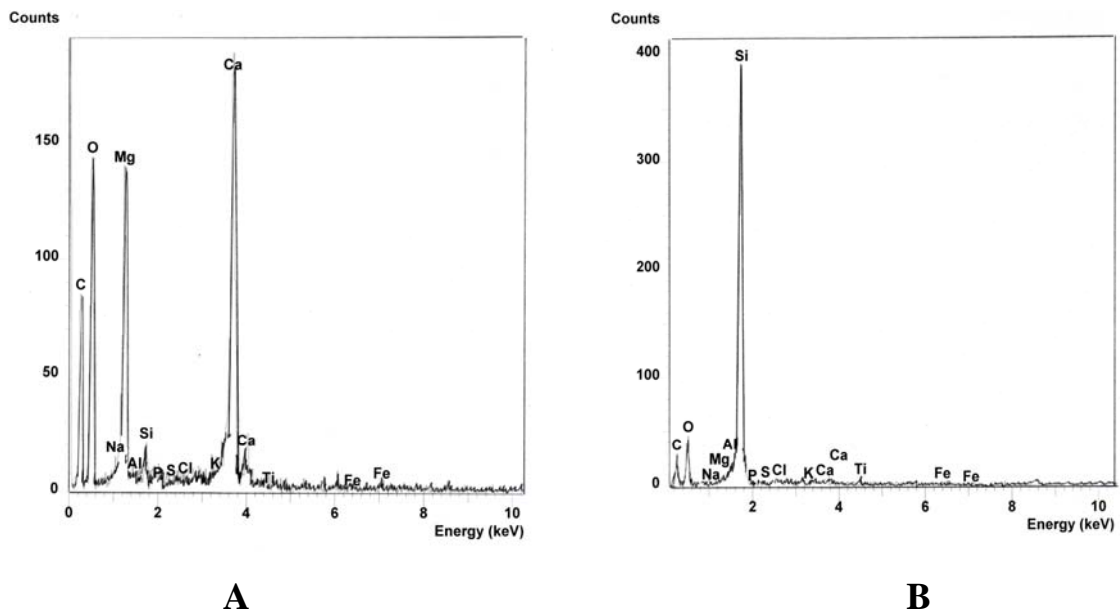
Fig. 5 EDS of sample no 8 - burnt material from fireplace. A – EDS of secondary crystallizing dolomite, B - EDS of Si-glass.
