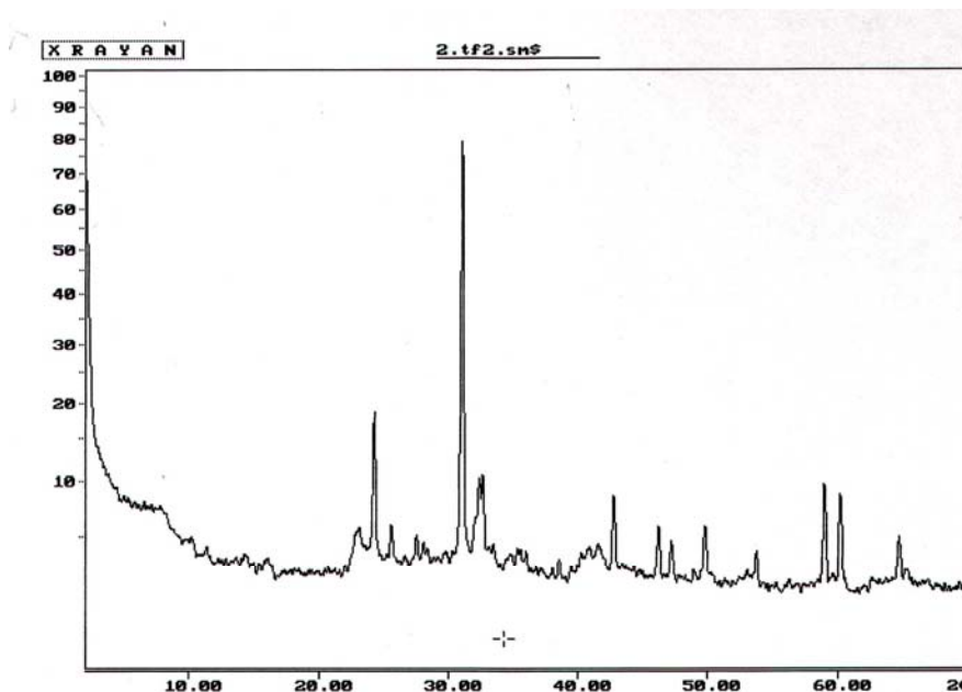
Fig. 2 X-ray pattern of yellowish clay containing clay minerals, quartz and traces of feldspars.
