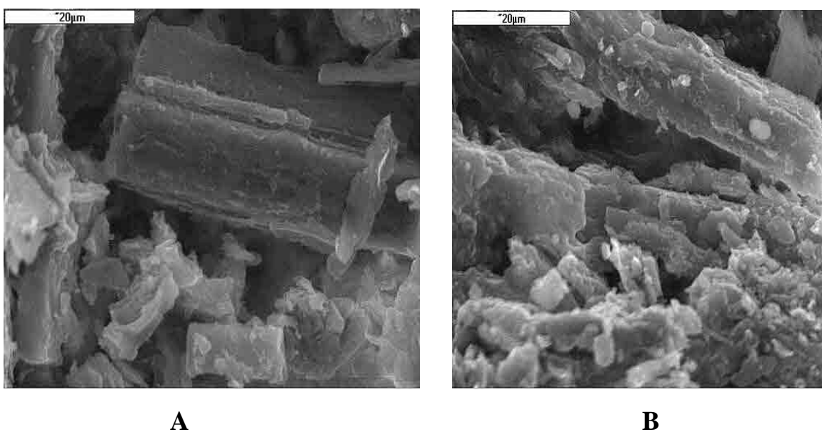
Photo 12. Sample no 9. A, B - fragments of mineralized mat surrounded by secondary minerals. SEM, magnification on scale.
