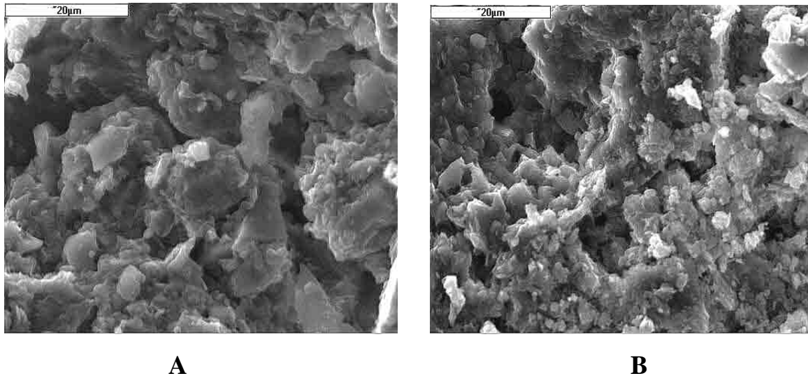
Photo 9. Sample no 5. Burnt grains of plant seen as irregular cracked structure (A) and small light grains of secondary aluminium silicates (B). SEM, magnification on scale.
