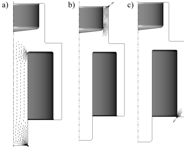
Fig. 8. Vectors of the metal displacement in final stage of extrusion process for lubrication variants: a) 1, 2, 4÷7; b) 8 i 9; c) 3
