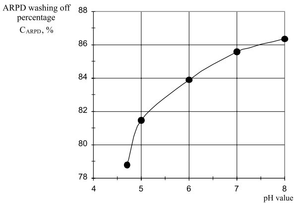
Fig. 2 . The dependence of the ARPD washing off percentage on the pH value at the time of the laboratory tests 12 hours and the temperature of 20°C for the well No 2
