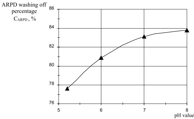
Fig. 1. The dependence of the ARPD washing off percentage on the pH value at the time of the laboratory tests 12 hours and the temperature of 20°C for the well No 1
