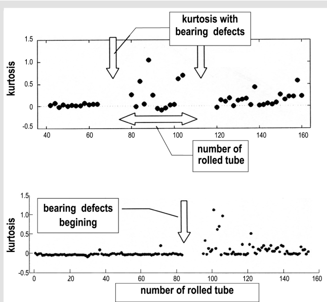
Fig. 5. Kurtosis of a vibration signal from a bearing in a pilger mill when the bearing track gets damaged
