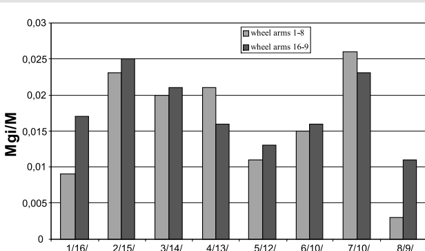
Fig. 4. Contributions of individual wheel arms to the transmission of inertia force moment. Condition after one year of service
