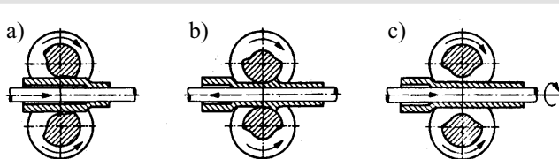
Fig. 1. Operating principle of a pilger mill (schematic diagram) a) reduction of wall thickness; b) wall calibration; c) tube release
