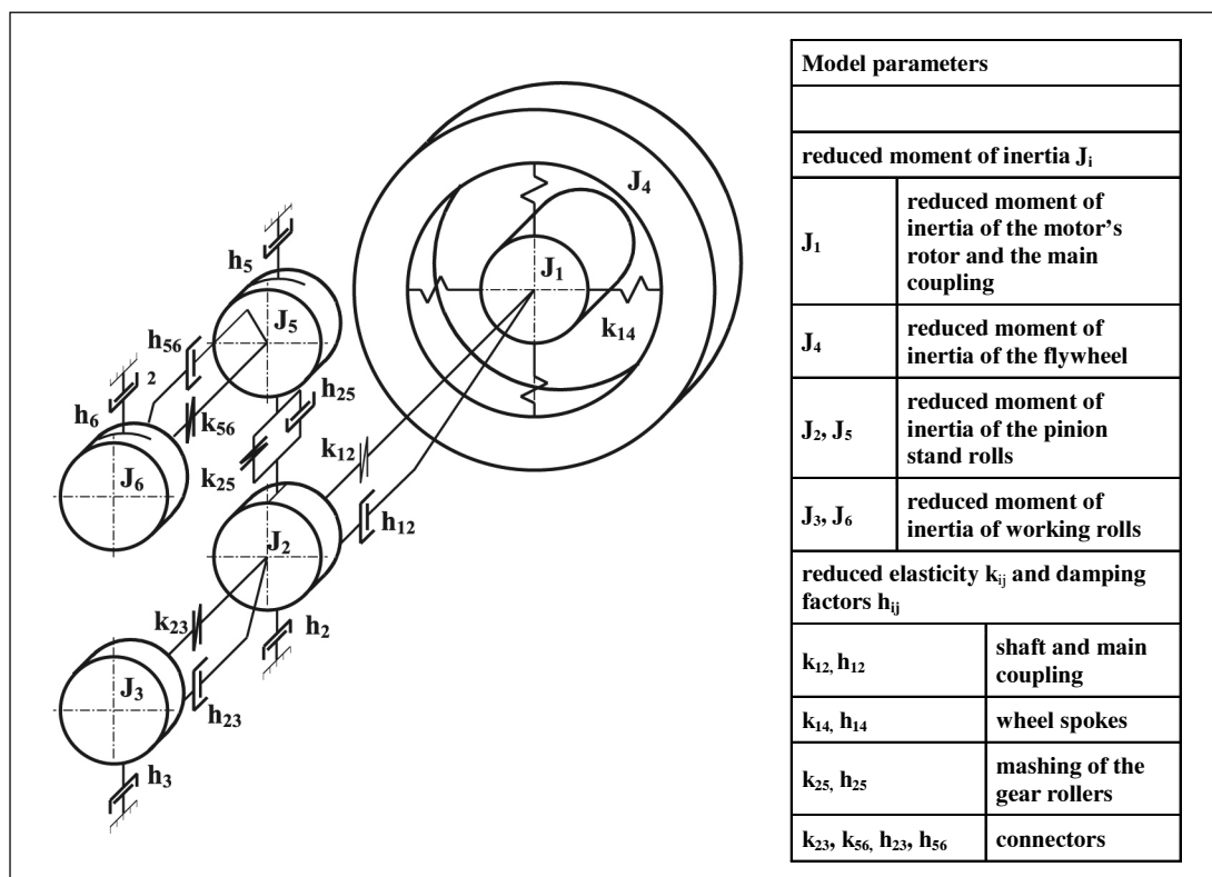
Fig. 6. Mass spring model of a pilger mill's drive reduced to a 6-DOF system
