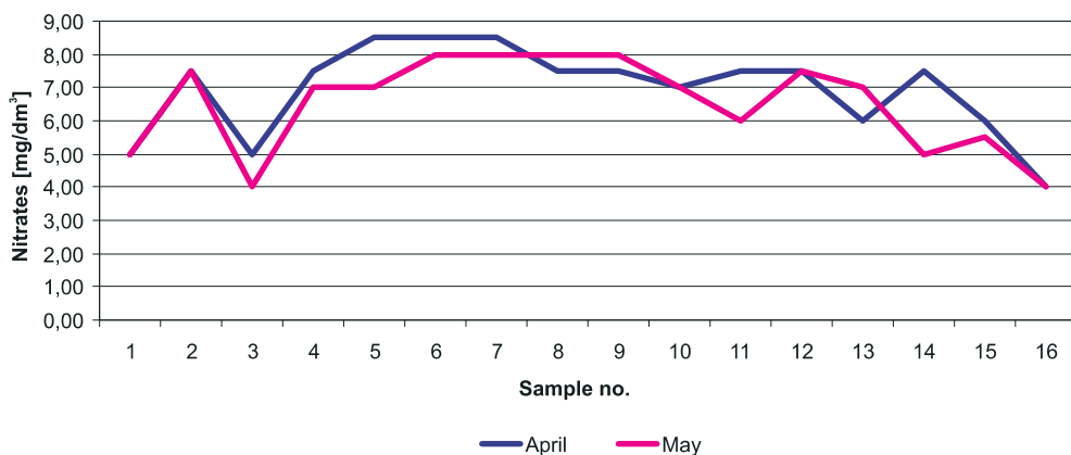
Fig. 3. The level of nitrates – spring
