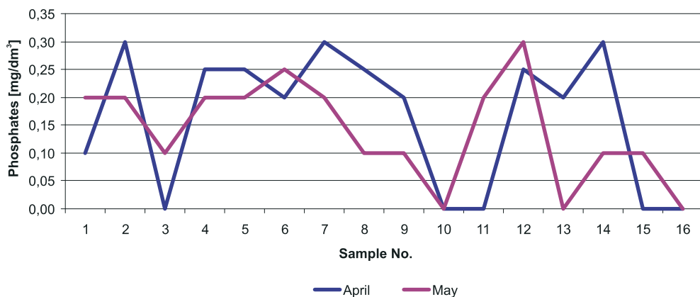
Fig. 4. The level of phosphates – spring
