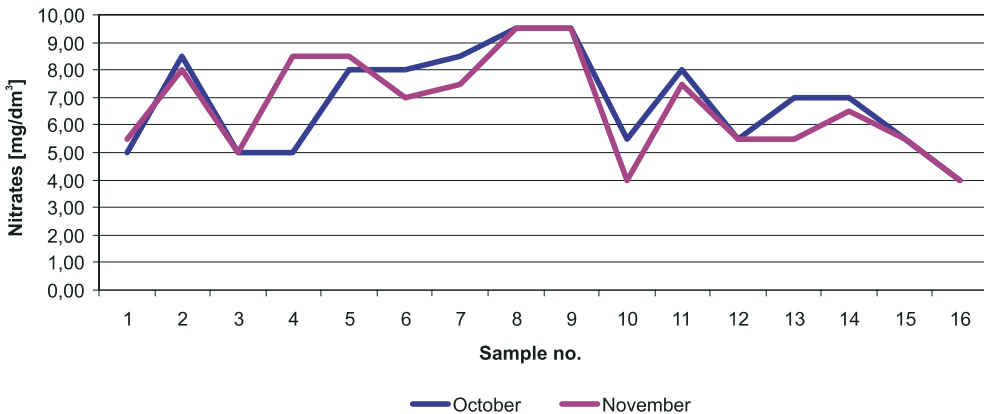
Fig. 5. The level of nitrates – autumn
