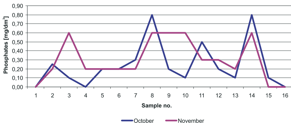
Fig. 6. The level of phosphates – autumn
