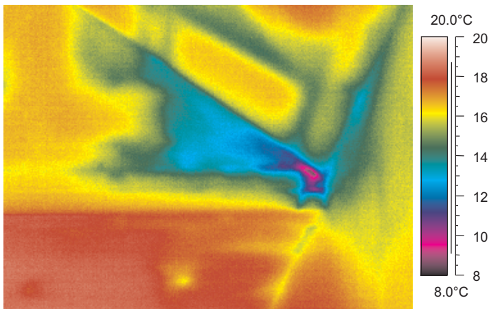
Fig. 1. Thermogram of the inner surface of the building outer walls conducted on 8.02.2008 at approximately 23:00, with the outdoor air temperature of 0°C
