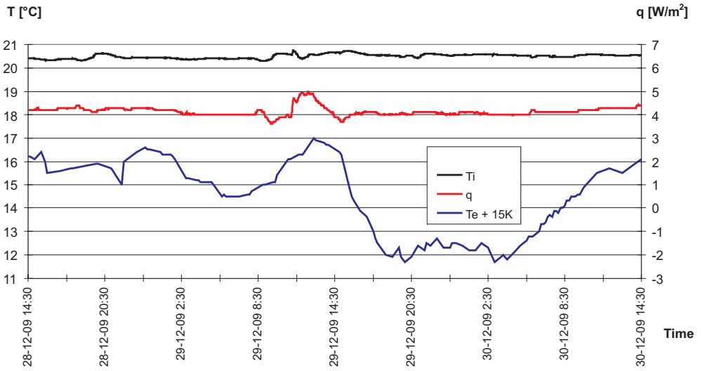
Fig. 6. The air temperature inside and outside of a multifamily building and the heat flux density with a stable central heating
