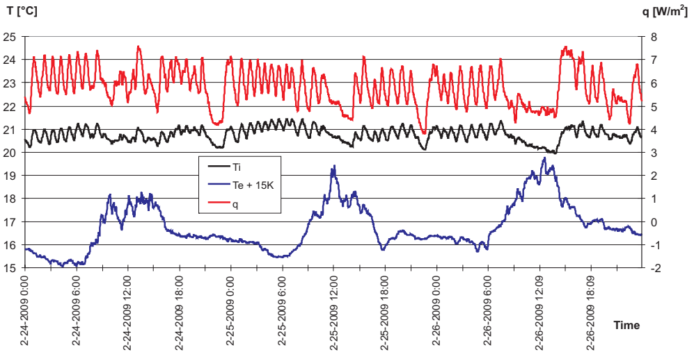
Fig. 4. The air temperature inside and outside of a single-family building and the heat flux density with central heating with automatic control
