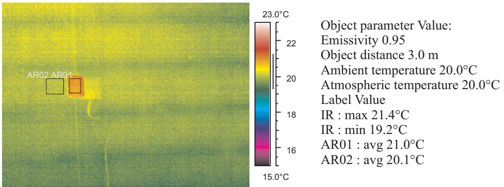
Fig. 8. Method of measuring air temperature and wall surface with thermographic method
