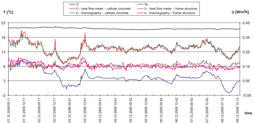
Fig. 9. The course of wall examination of an actual building
