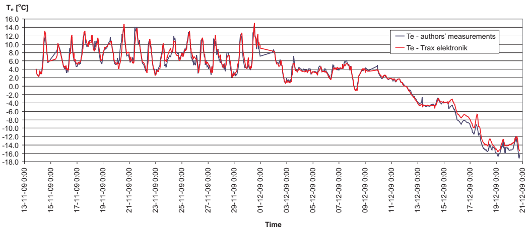
Fig. 3. Outside air temperature measured at the examined building and at a road weather station located at a distance of 1 km from the building
