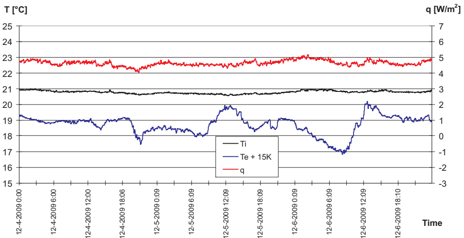
Fig. 5. The air temperature inside and outside of a single-family building and the heat flux density with a steady electrical heating
