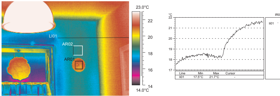
Fig. 2. Thermogram of the inner surface of the outer wall conducted on 3.01.2010 at approximately 20:00, with the outdoor air temperature of -8.0^{\circ}\text{C}
