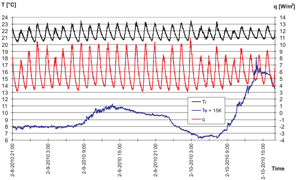
Fig. 7. The air temperature inside and outside of a multifamily building and the heat flux density with automatic regulation of central heating
