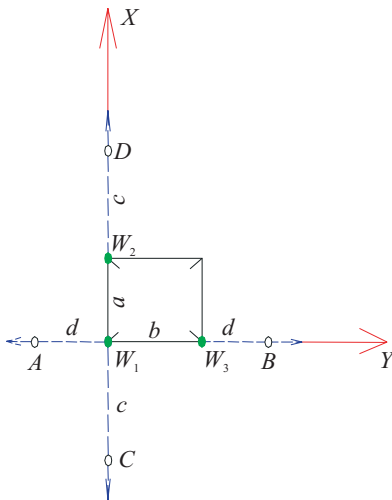
Fig. 3. Determining of not easily accessible terrain details with the use of an indirect measure method – straight line intersection
