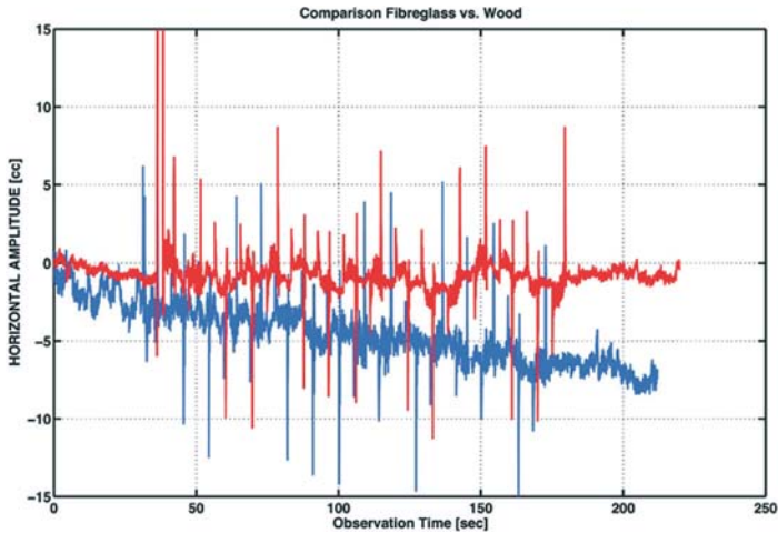
Fig. 3. Hz-Stability of fibreglass compared to a wooden model
