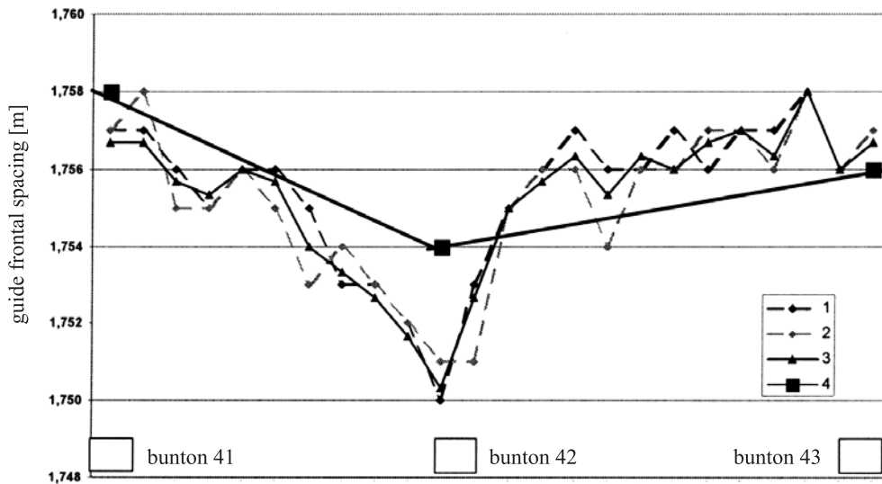
Fig. 6. Guide front spacing between buntuns 41–43 (1–3 – measurements taken with DISTO plus, 4 – conventional measurement)
