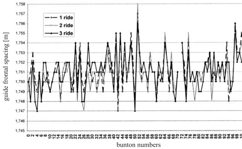
Fig. 4. Frontal spacing between two guides (values obtained in three rides)
