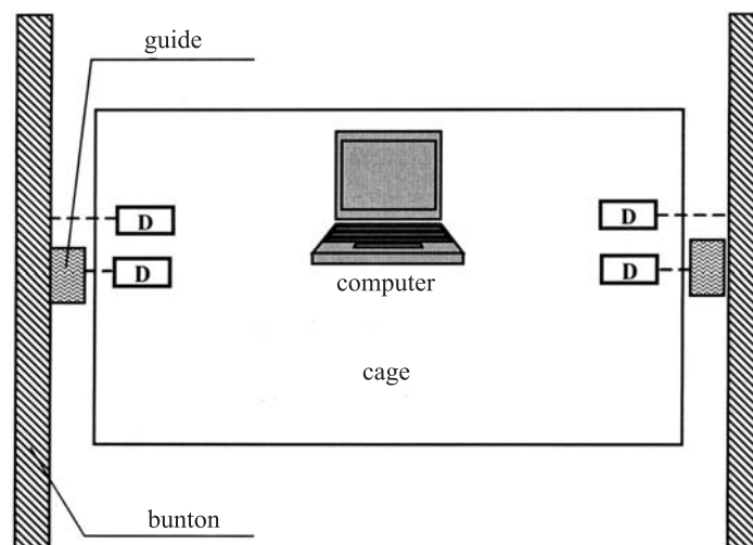
Fig. 2. Layout of the measuring equipment in a cage, configured to measure guide and bunton spacing
