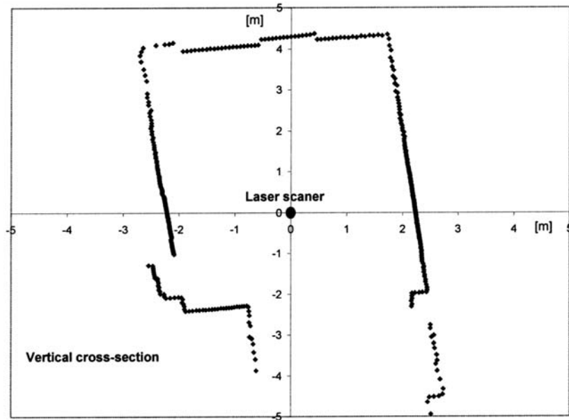
Fig. 10. Horizontal cross-section of the corridor (in the building C-4) obtained with the use of a laser scanner
