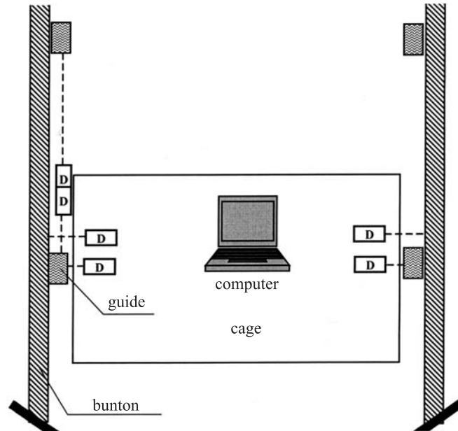
Fig. 3. Layout of the measuring equipment in a cage, configured to measure the guide frontal and lateral spacing and the bunton spacing
