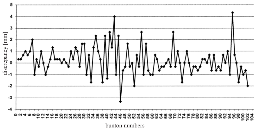
Fig. 5. Differences between the measured guide spacing value obtained by the conventional method and with the use of DISTO plus distancemeters
