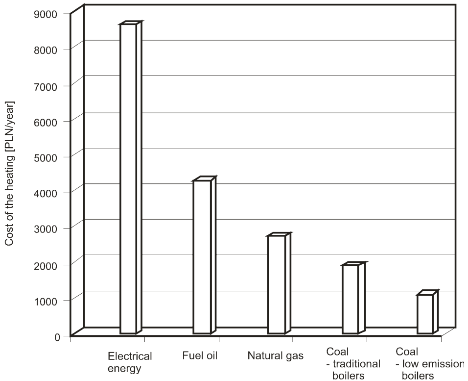
Fig. 1. Example — cost of heating of the room with the surface 100 m 2 at the use of different types of energy and technologies of combustion
