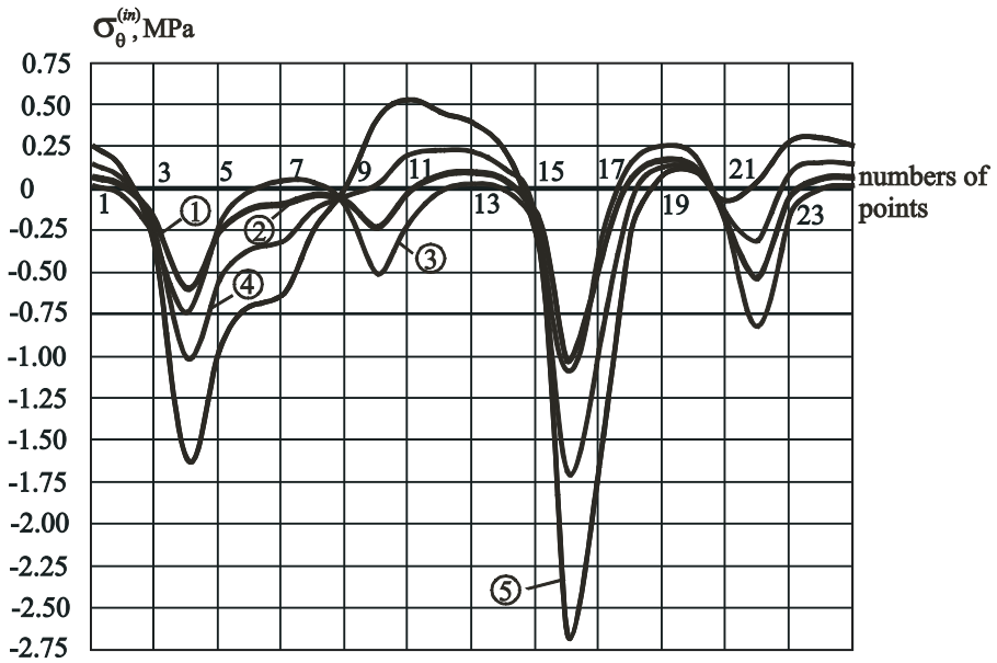
Fig. 4. Stresses \sigma_{\theta}^{(in)} in points of the internal lining outline (see text)
