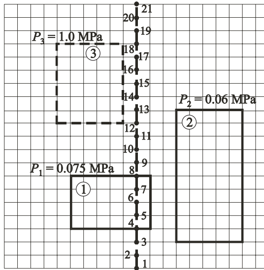
Fig. 3. Plan of building locations
