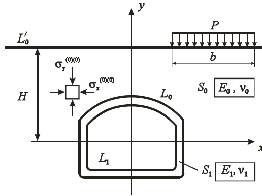
Fig. 1. The design scheme
