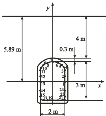
Fig. 2. The lining cross-section
