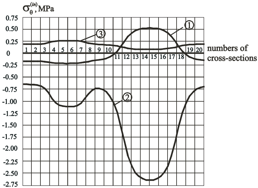
Fig. 5. Changing of stresses \sigma_{\theta}^{(in)} in points 11, 16, 19 along the tunnel length (see text)
