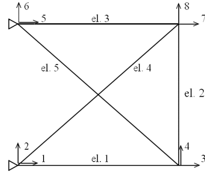
Fig. 1. Truss structure testing example
