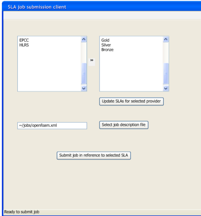
Figure 6. SLA selection and job submission using a GUI client.
