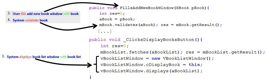
Figure 10. Dynamic code generated for SVO sentences.
