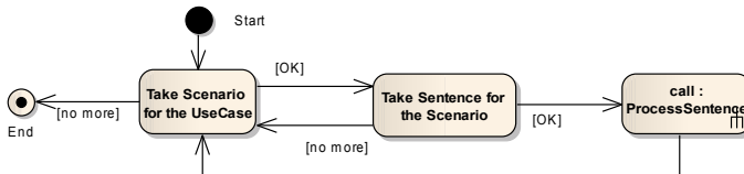
Figure 13. General algorithm for use case processing.
