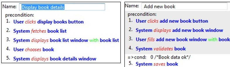
Figure 2. Concrete syntax for use case scenarios.
