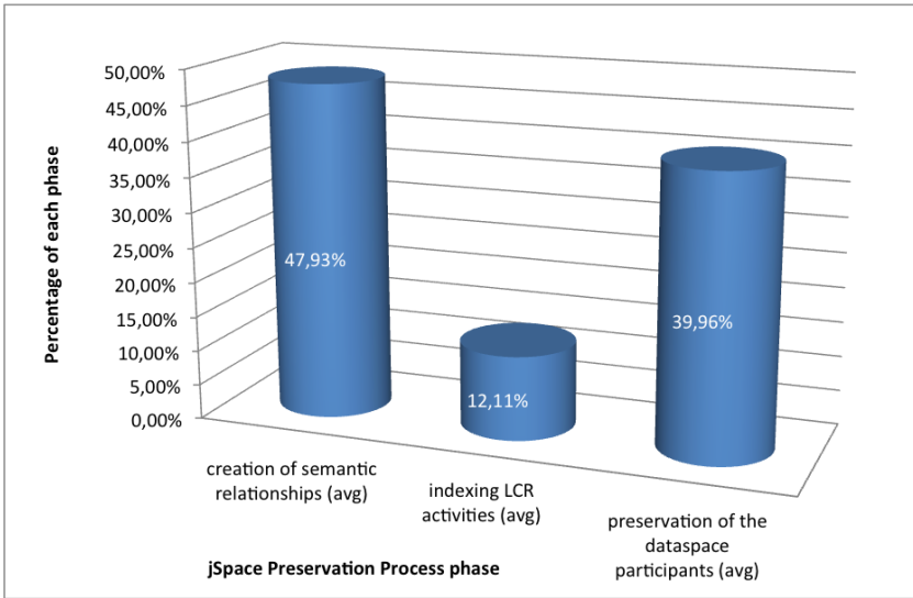
Figure 3. Distribution of the performance overhead among the phases of the jSpace PP (average on preservation of 100 NIGM-LCRs)
