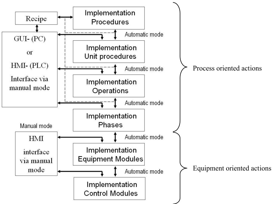
Fig. 3. Recipe driven automatic mode and manual mode as an alternative during development following the Bottom-Up approach
