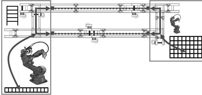
Fig. 4. Storage unit (right) and formation unit (left) are handling the material flow independent
