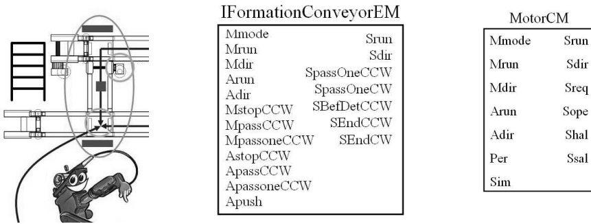
Fig. 6. Example of an EM: The Formation Conveyor Equipment Module, which is formed by 2 Motor CMs (circles), 2 rockerstop CMs (rectangles) and a stopgate CM (square)
