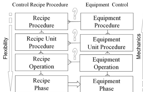
Fig. 5. The level of linking recipe and equipment control
