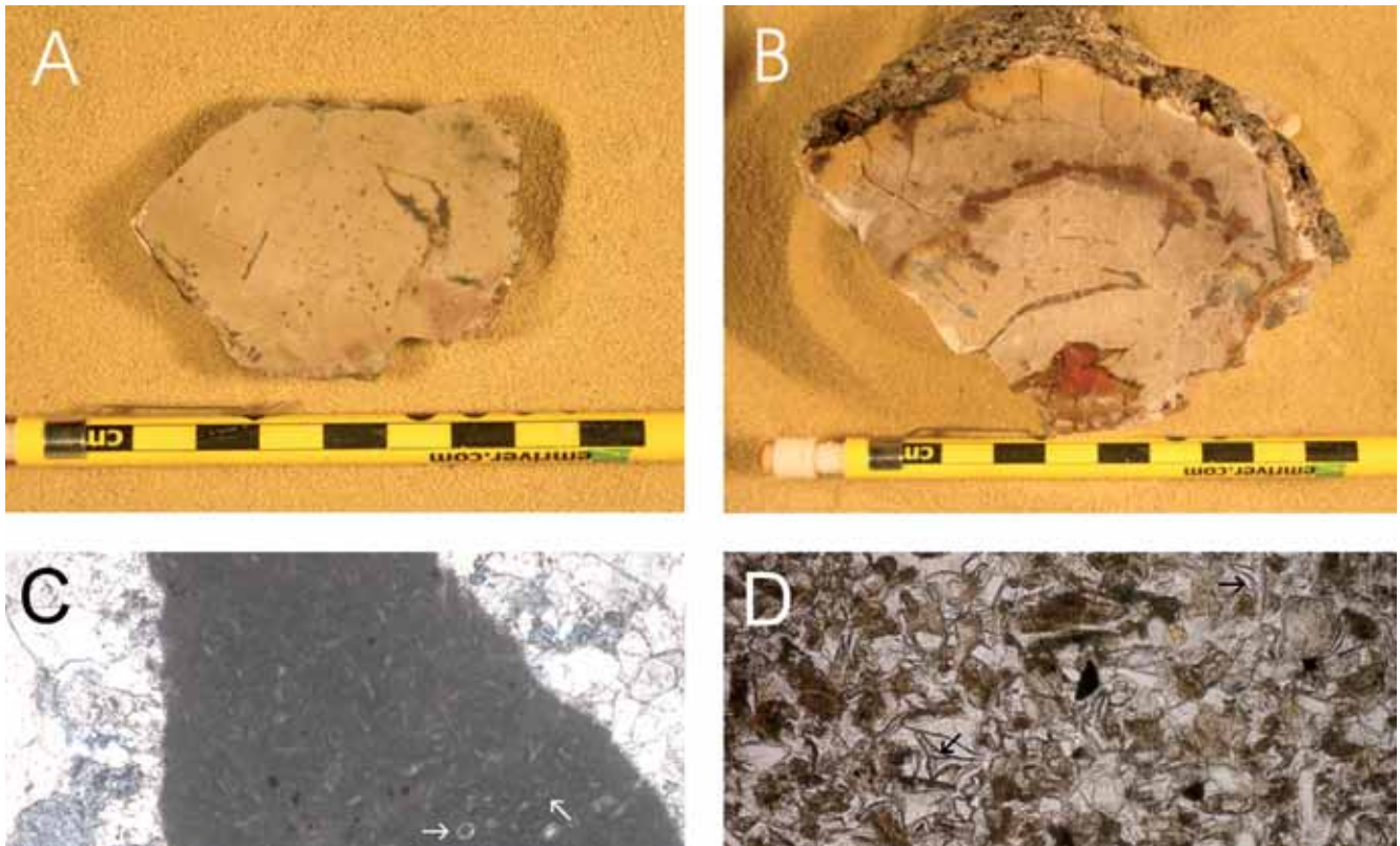
Fig. 7. Features of Brushy Basin limestones
