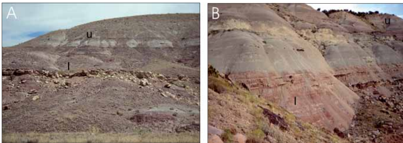
Fig. 2. Differences between lower (l) and upper (u) Brushy Basin Member lithologies
