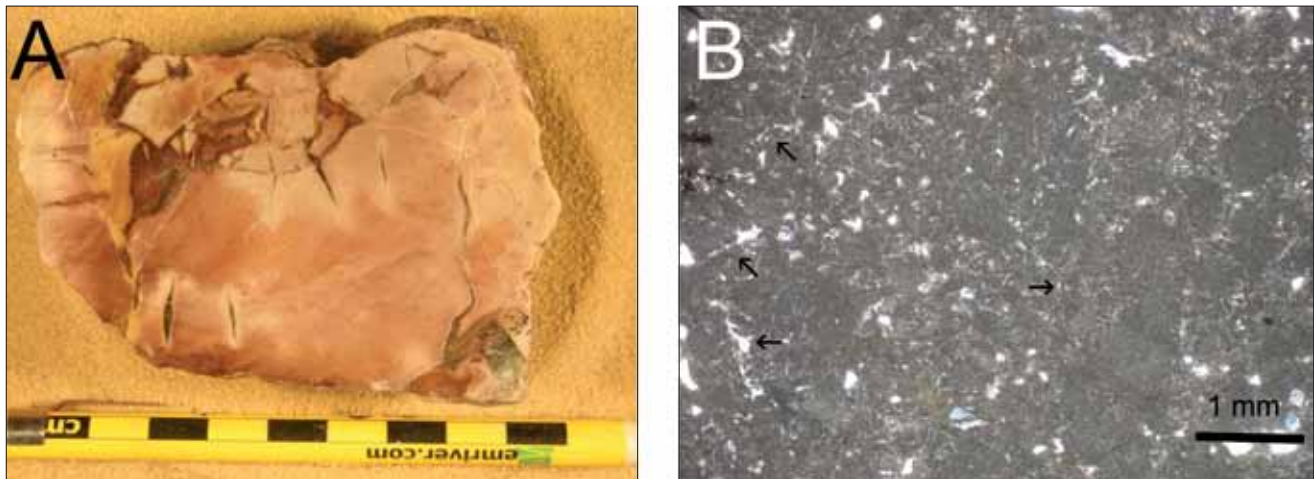
Fig. 8. Palustrine limestone features
