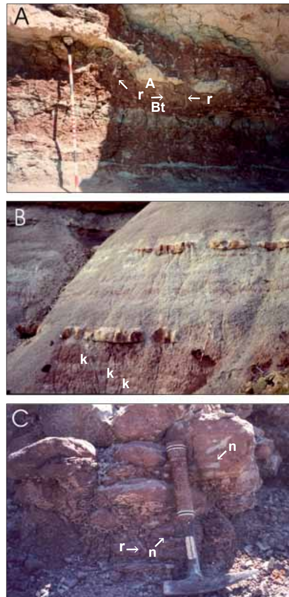
Fig. 3. Features of lower Brushy Basin Member paleosols
