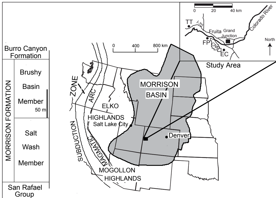
Fig. 1. Map depicting limits of the extent of Morrison Formation deposition, location of the area of this study relative to the Morrison depositional basin, and stratigraphy of the study area modified from Galli (2014 – this volume)
