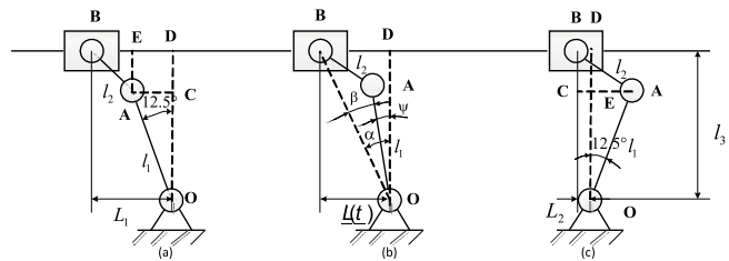
Fig. 5 Mechanism Moment Position
