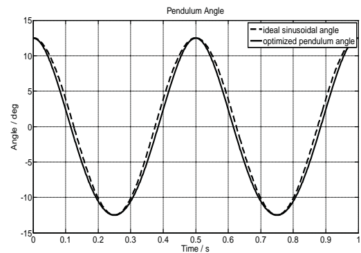
Fig. 7 The output angle of the mechanism and the ideal output angle
