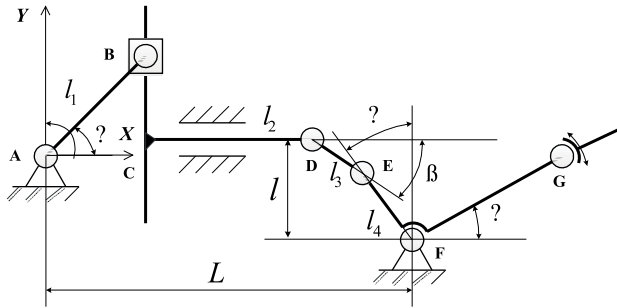
Fig. 3 The mechanism sketch of the propulsion mechanism
