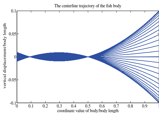
Fig. 1 The centerline trajectories of the fish body
