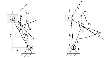
Fig. 6 The transmission angle at the limit position \theta_1
