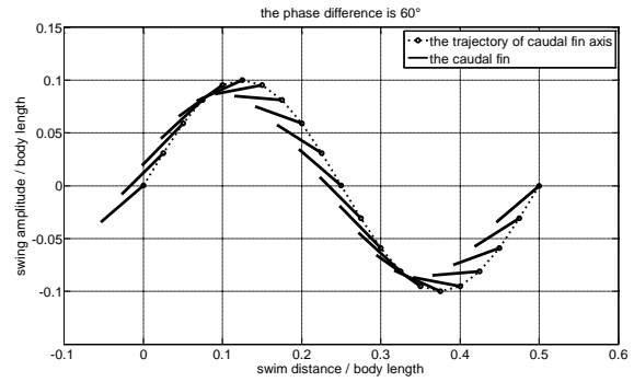
Fig. 9 The phase difference is 60^\circ
