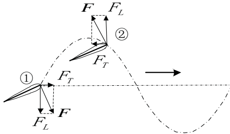
Fig. 8 Analysis of the forces on caudal fin
