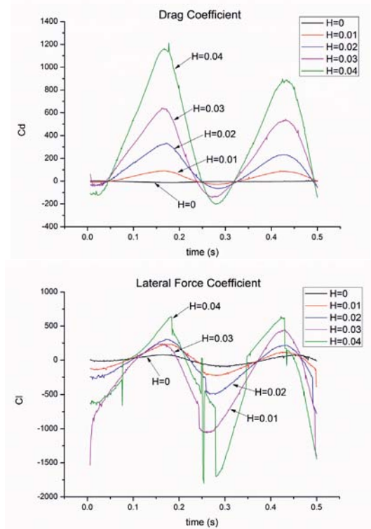
Fig. 12 Drag coefficient curves and lateral force coefficient curves of fish body in the still water
