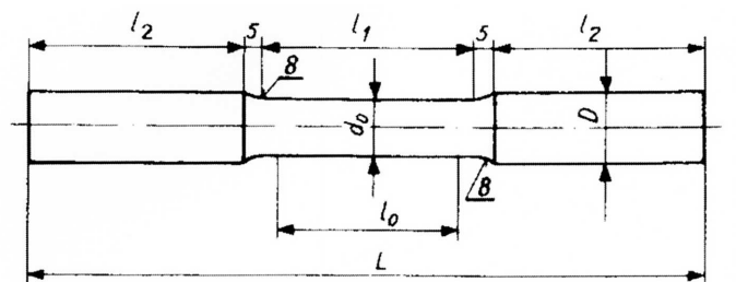
Fig. 1. Specimen geometry used in tests
