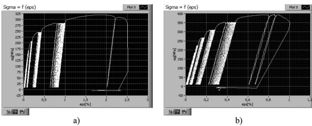
Fig. 2. The σ = f(ε) curve for G20Mn5 cast steel; a) specimen 5.2, b) specimen 5.3
