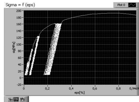
Fig. 3. The σ = f(ε) curve for G20Mn5 cast steel; specimen 5.5
