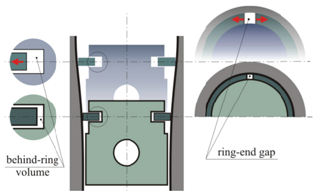
Fig. 2. Effect of cylinder deformations upon cross-section area of ring lock and behind-ring space
