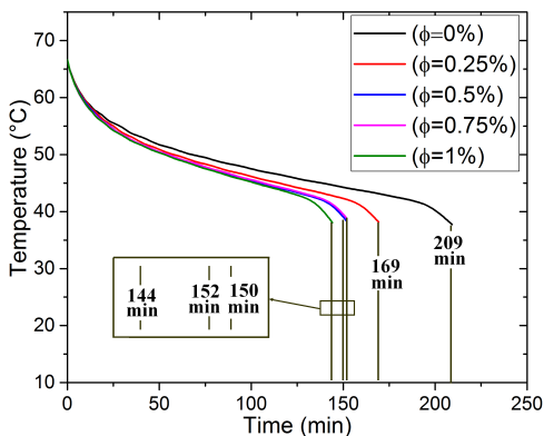
Fig. 13. The total average temperature of the HNPCM samples during discharging process
