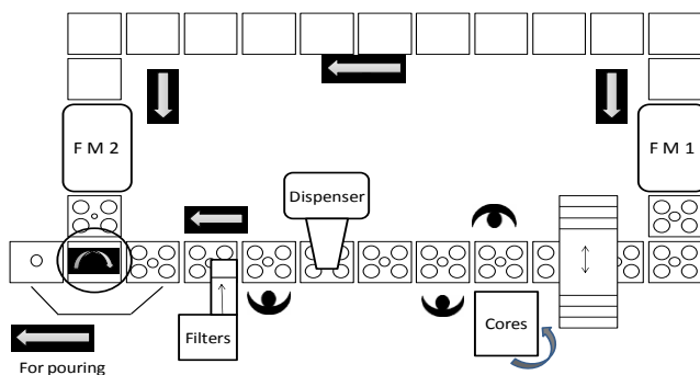
Fig. 4. A fragment of automated casting line after changes
