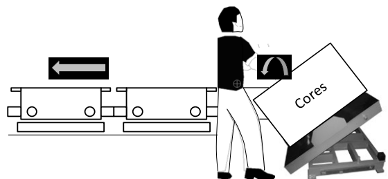
Fig. 6. Reorganization of the workplace of manual cores installation
