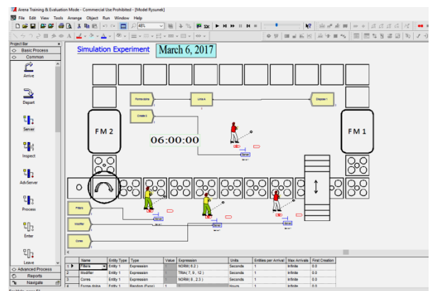
Fig. 5. A model of a casting line in the Arena software
