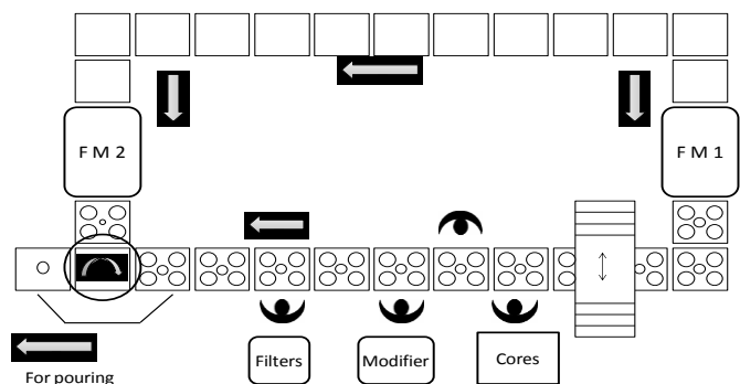
Fig. 2. A fragment of automated casting line before changes
