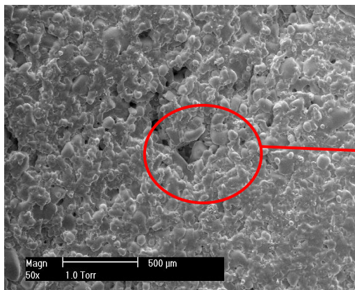
Fig. 5. SEM micrograph, 500–250 \mu\text{m} , 20% dry dextrin, 1 MPa, 700°C
