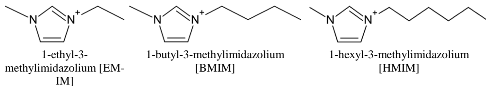
Fig. 1. Structure of ionic liquids cations used in the experiments
