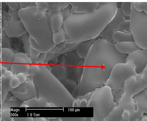
Fig. 6. SEM micrograph, 500–250 \mu\text{m} , 20% dry dextrin, MPa, 700°C
