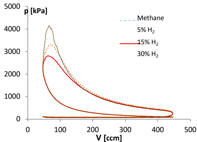
Fig. 2. Pressure changes in the p - V system, an engine Fueled with methane/hydrogen blends, n = 2500 rpm, WOT=100%, and \lambda = 1.0
