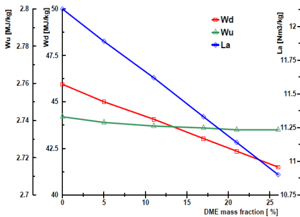
Fig. 7. Mass heating value as a function of DME mass ratio: W u – the mass heating value of a stoichiometric mixture, W d – the mass heating value of fuel, and L a – the stoichiometric air to fuel ratio
